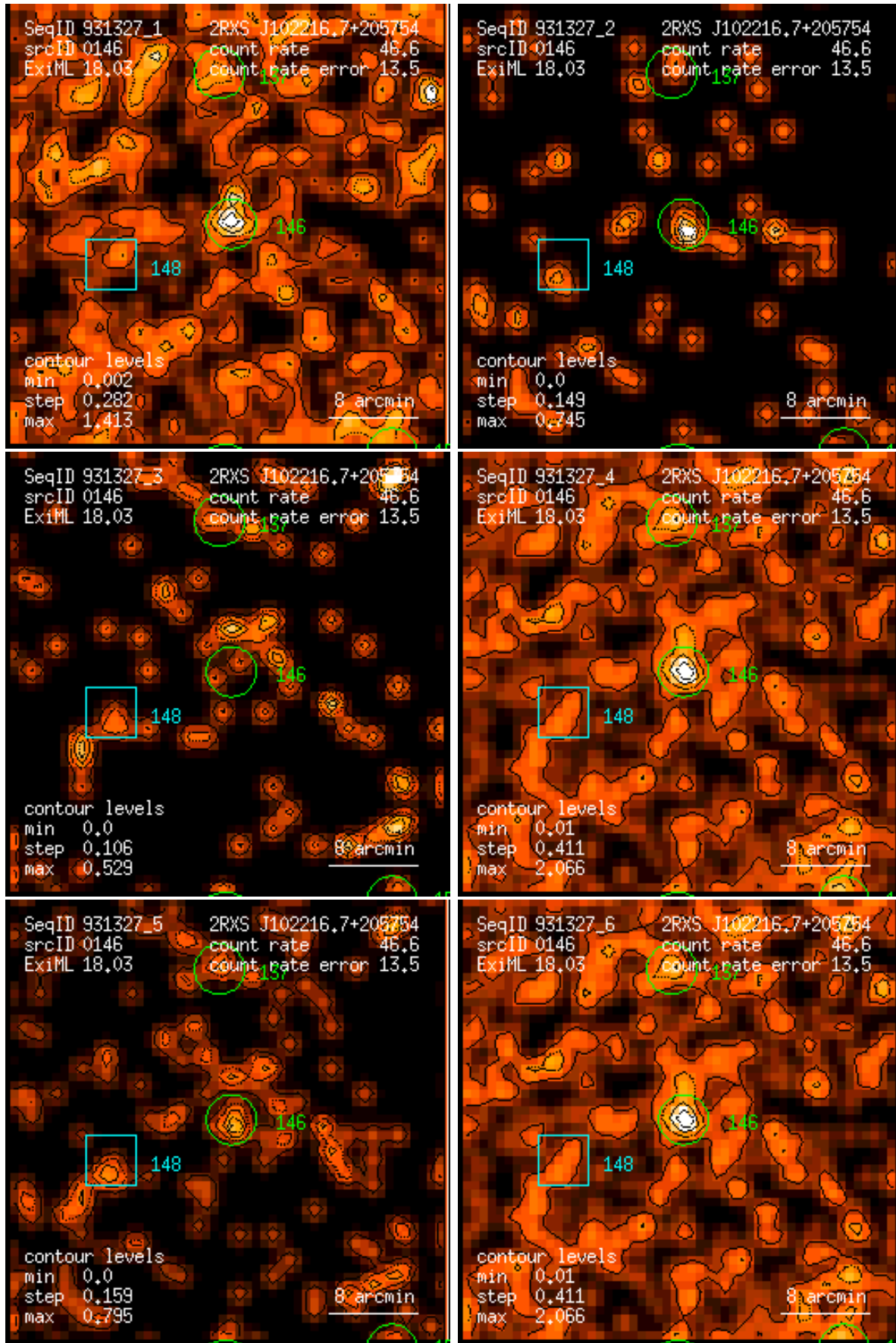
Figure 146: RASS 931327: detection 0146: band rate images, Gaussian filter: (1) PSPC channels 11 – 41, (2) 52 – 90, (3) 91 – 201, (4) 11 – 235, (5) 52 – 201, (6) 11 – 201. Broad band rates in counts/ks. Band rate contour levels in counts/ks/arcmin 2 .
