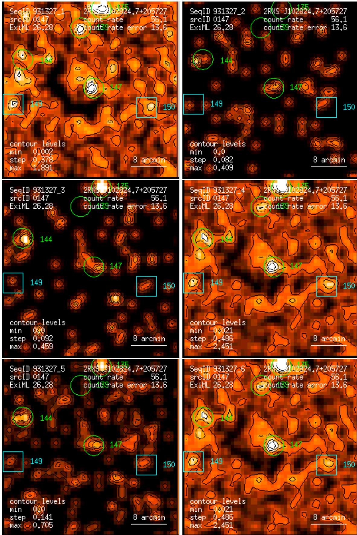
Figure 147: RASS 931327: detection 0147: band rate images, Gaussian filter: (1) PSPC channels 11 – 41, (2) 52 – 90, (3) 91 – 201, (4) 11 – 235, (5) 52 – 201, (6) 11 – 201. Broad band rates in counts/ks. Band rate contour levels in counts/ks/arcmin 2 .
