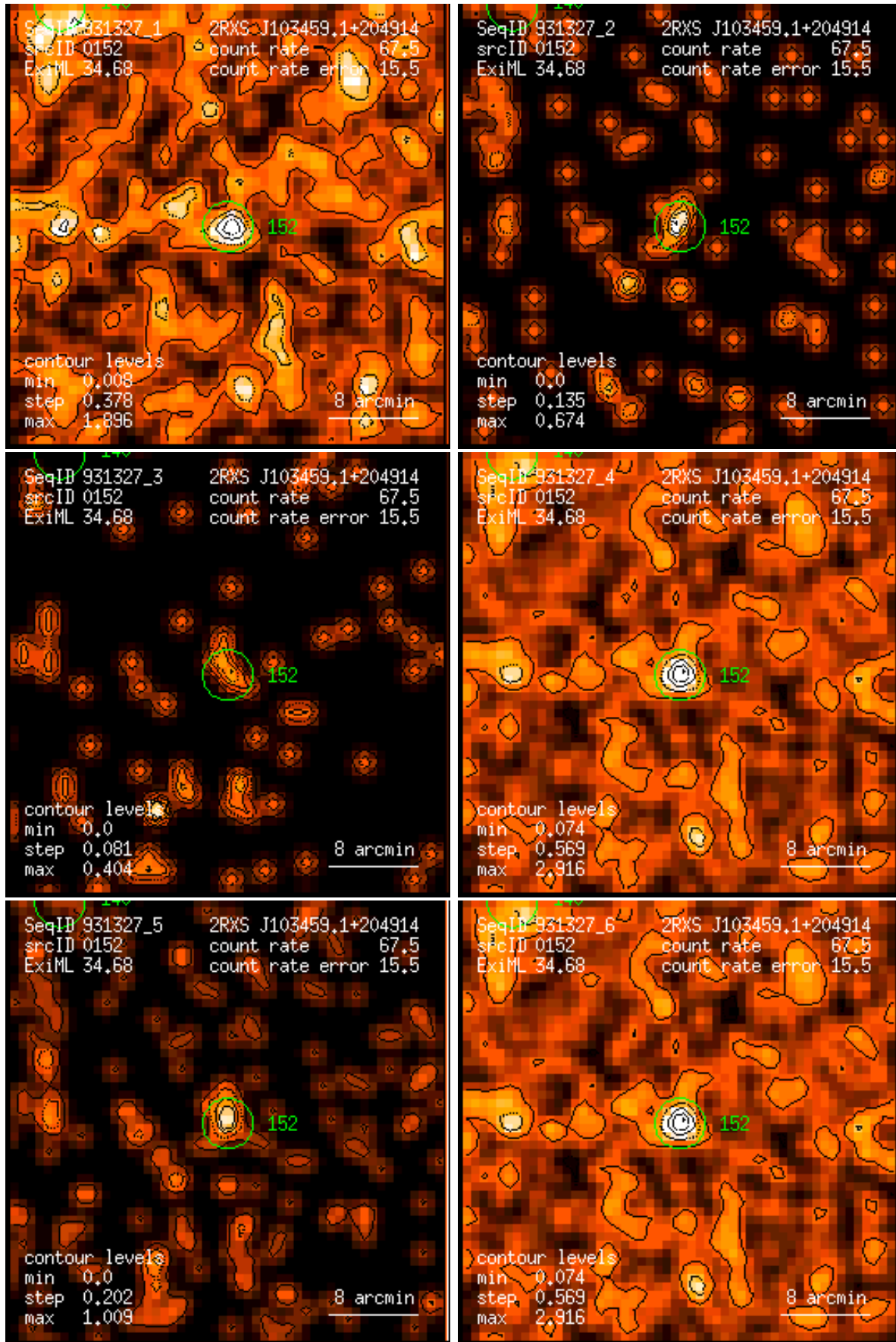
Figure 152: RASS 931327: detection 0152: band rate images, Gaussian filter: (1) PSPC channels 11 – 41, (2) 52 – 90, (3) 91 – 201, (4) 11 – 235, (5) 52 – 201, (6) 11 – 201. Broad band rates in counts/ks. Band rate contour levels in counts/ks/arcmin 2 .
