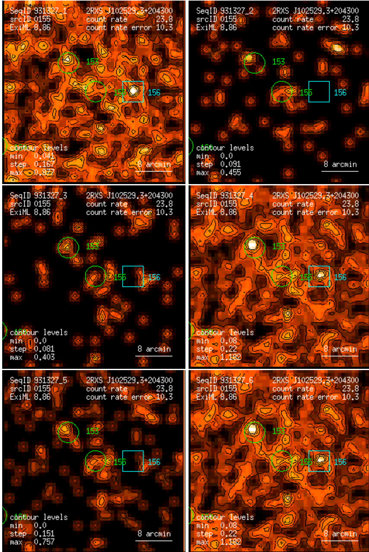
Figure 155: RASS 931327: detection 0155: band rate images, Gaussian filter: (1) PSPC channels 11 – 41, (2) 52 – 90, (3) 91 – 201, (4) 11 – 235, (5) 52 – 201, (6) 11 – 201. Broad band rates in counts/ks. Band rate contour levels in counts/ks/arcmin 2 .
