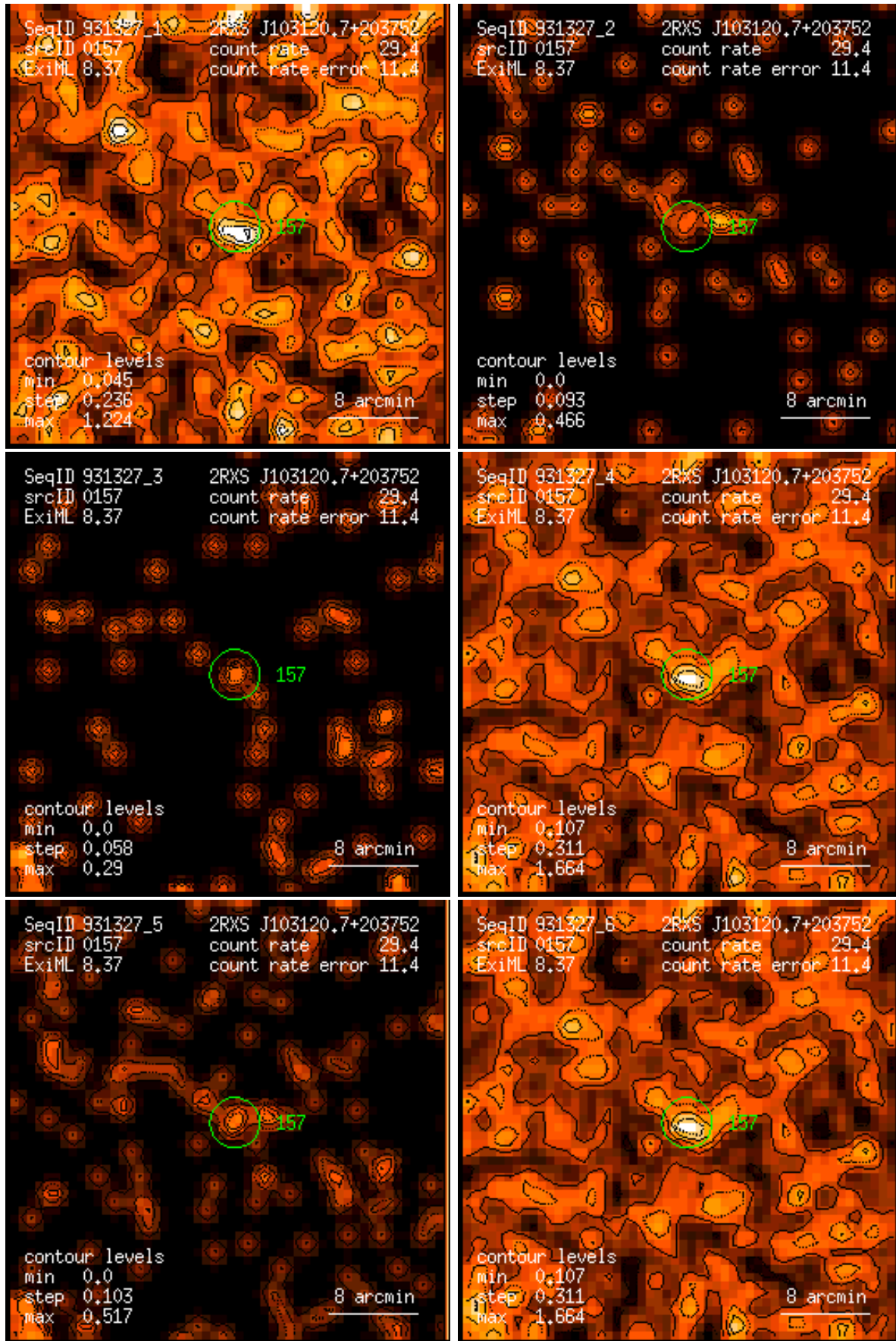
Figure 157: RASS 931327: detection 0157: band rate images, Gaussian filter: (1) PSPC channels 11 – 41, (2) 52 – 90, (3) 91 – 201, (4) 11 – 235, (5) 52 – 201, (6) 11 – 201. Broad band rates in counts/ks. Band rate contour levels in counts/ks/arcmin 2 .
