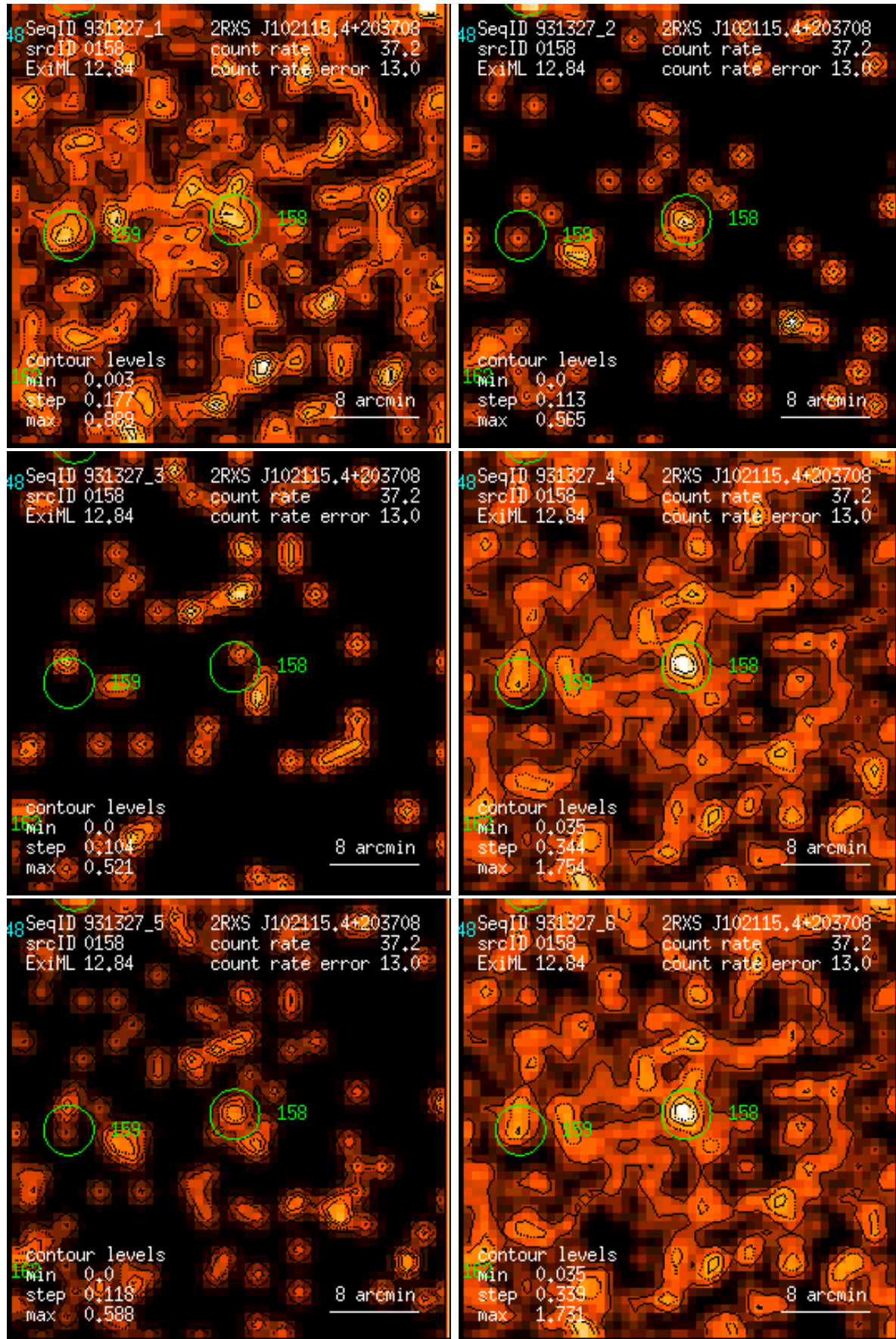
Figure 158: RASS 931327: detection 0158: band rate images, Gaussian filter: (1) PSPC channels 11 – 41, (2) 52 – 90, (3) 91 – 201, (4) 11 – 235, (5) 52 – 201, (6) 11 – 201. Broad band rates in counts/ks. Band rate contour levels in counts/ks/arcmin 2 .
