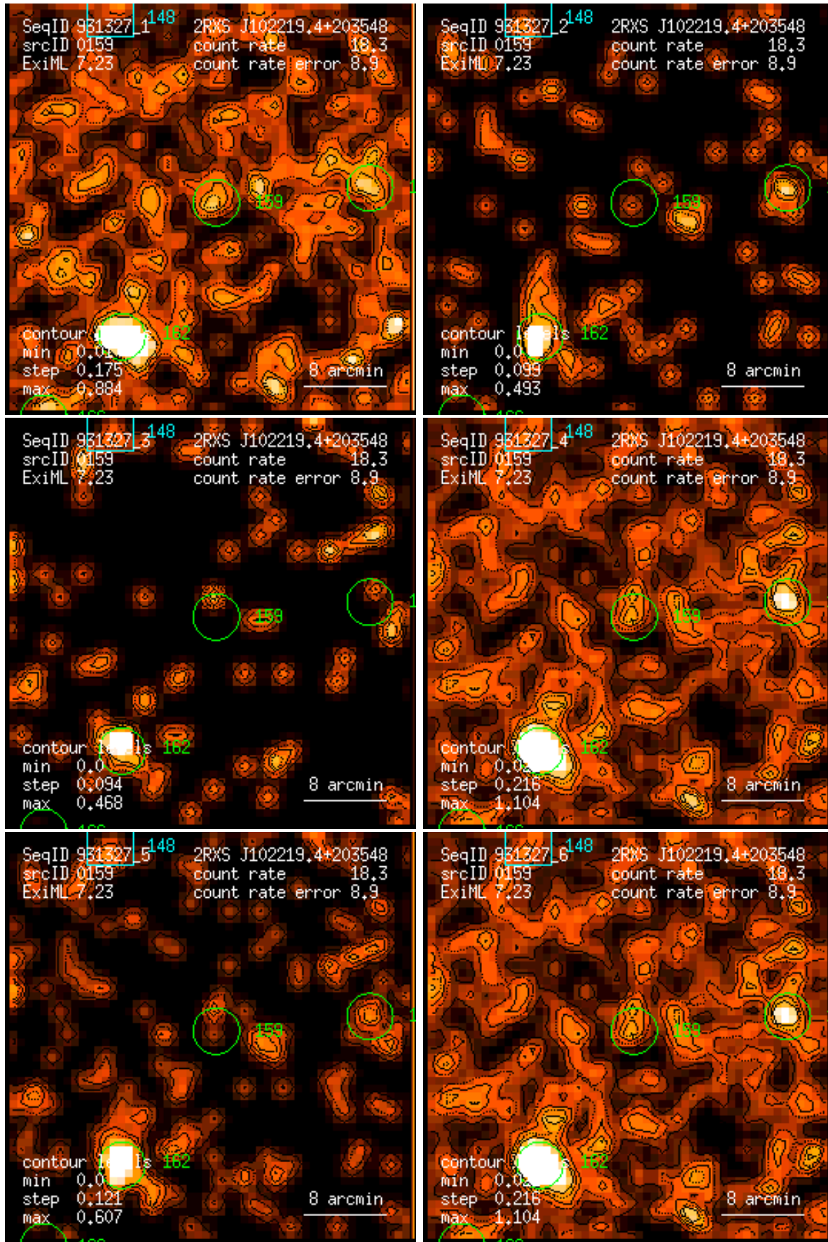
Figure 159: RASS 931327: detection 0159: band rate images, Gaussian filter: (1) PSPC channels 11 – 41, (2) 52 – 90, (3) 91 – 201, (4) 11 – 235, (5) 52 – 201, (6) 11 – 201. Broad band rates in counts/ks. Band rate contour levels in counts/ks/arcmin 2 .
