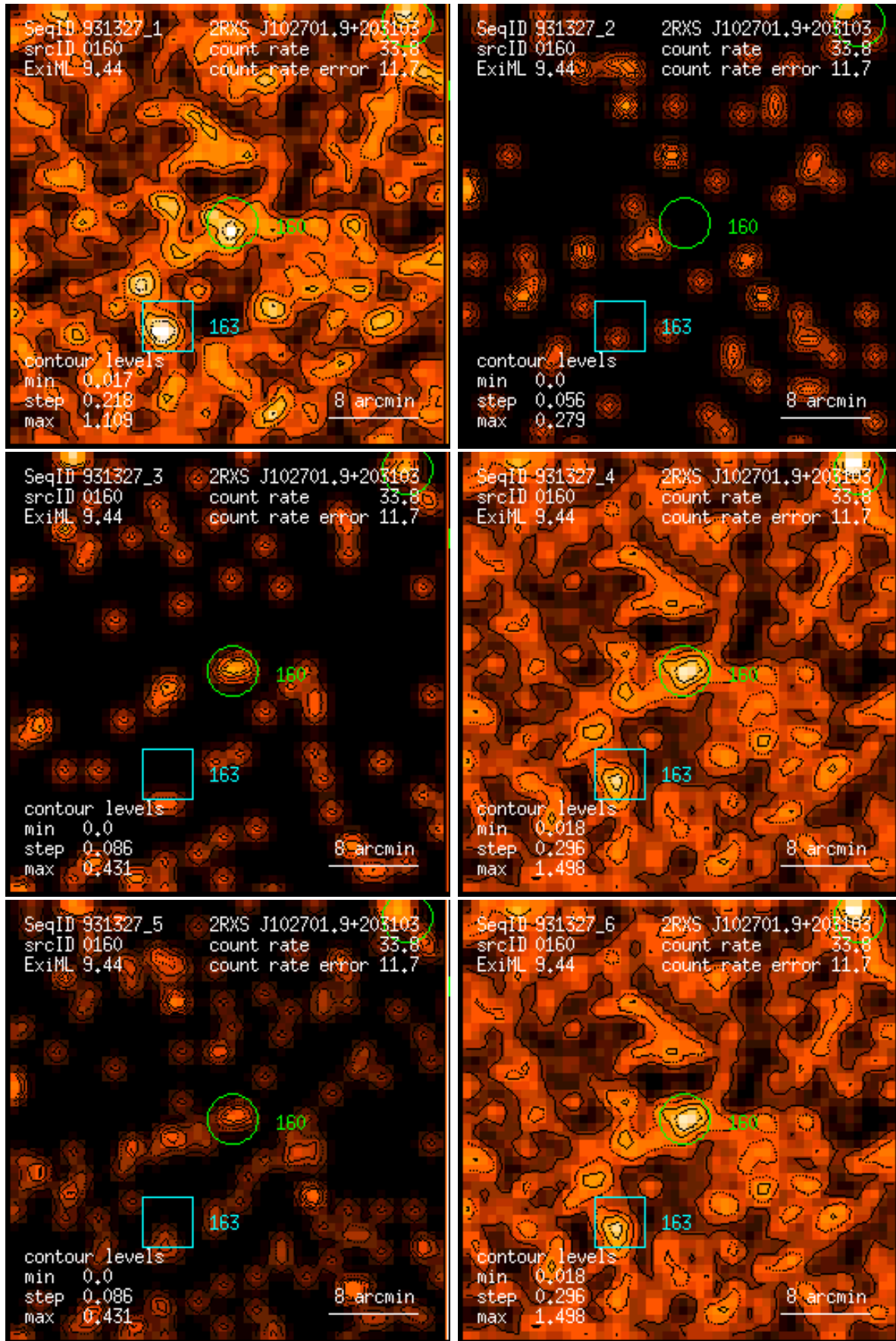
Figure 160: RASS 931327: detection 0160: band rate images, Gaussian filter: (1) PSPC channels 11 – 41, (2) 52 – 90, (3) 91 – 201, (4) 11 – 235, (5) 52 – 201, (6) 11 – 201. Broad band rates in counts/ks. Band rate contour levels in counts/ks/arcmin 2 .
