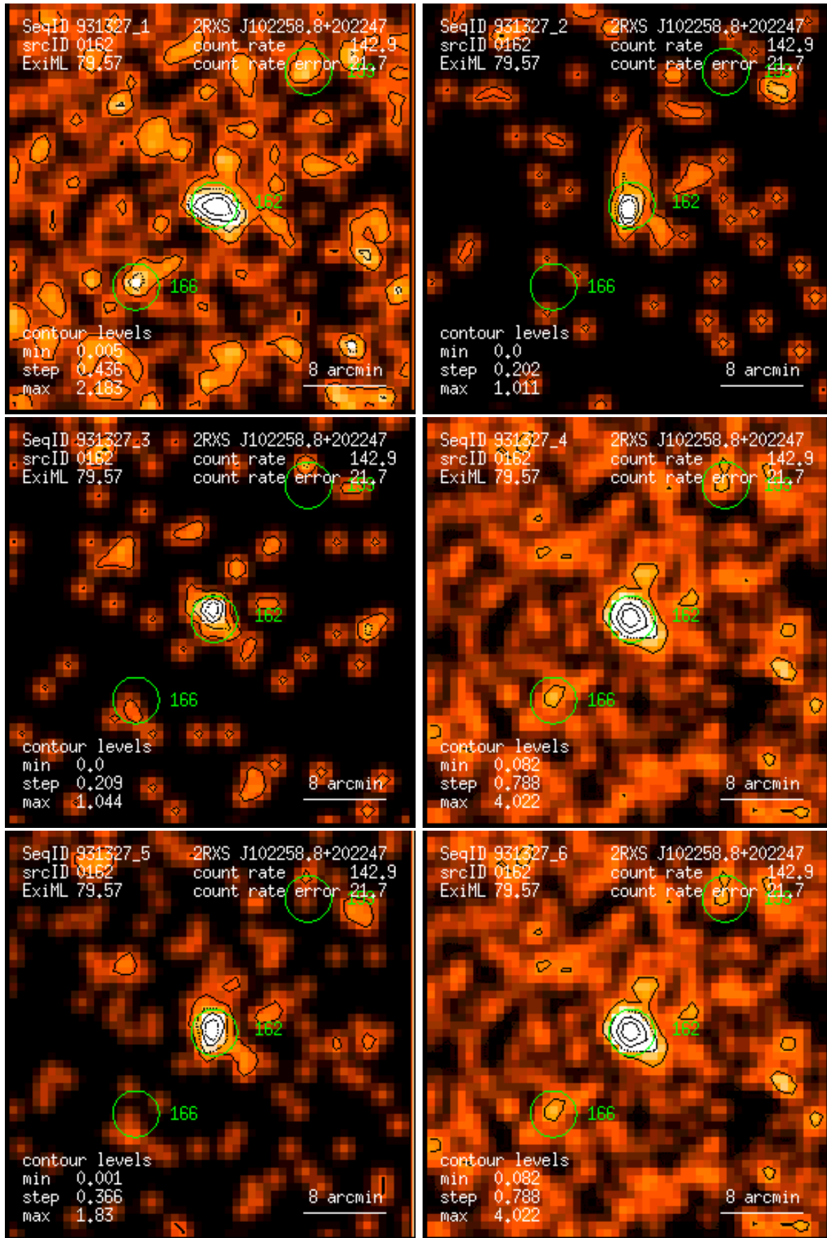
Figure 162: RASS 931327: detection 0162: band rate images, Gaussian filter: (1) PSPC channels 11 – 41, (2) 52 – 90, (3) 91 – 201, (4) 11 – 235, (5) 52 – 201, (6) 11 – 201. Broad band rates in counts/ks. Band rate contour levels in counts/ks/arcmin 2 .
