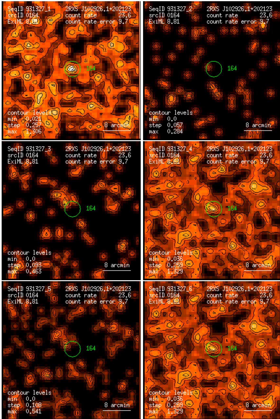
Figure 164: RASS 931327: detection 0164: band rate images, Gaussian filter: (1) PSPC channels 11 – 41, (2) 52 – 90, (3) 91 – 201, (4) 11 – 235, (5) 52 – 201, (6) 11 – 201. Broad band rates in counts/ks. Band rate contour levels in counts/ks/arcmin 2 .
