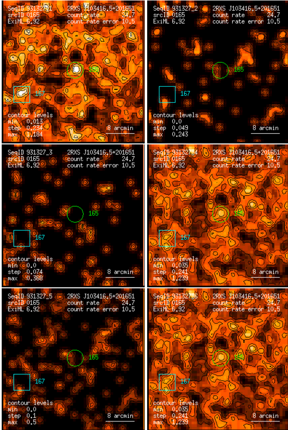
Figure 165: RASS 931327: detection 0165: band rate images, Gaussian filter: (1) PSPC channels 11 – 41, (2) 52 – 90, (3) 91 – 201, (4) 11 – 235, (5) 52 – 201, (6) 11 – 201. Broad band rates in counts/ks. Band rate contour levels in counts/ks/arcmin 2 .
