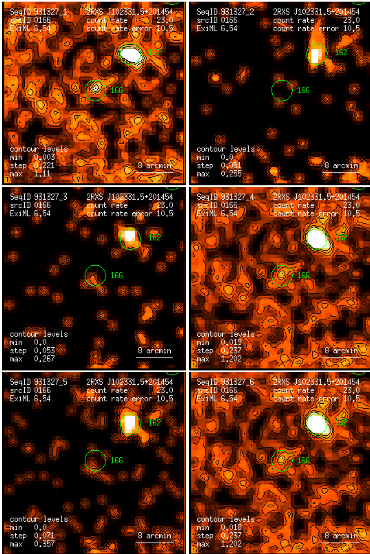
Figure 166: RASS 931327: detection 0166: band rate images, Gaussian filter: (1) PSPC channels 11 – 41, (2) 52 – 90, (3) 91 – 201, (4) 11 – 235, (5) 52 – 201, (6) 11 – 201. Broad band rates in counts/ks. Band rate contour levels in counts/ks/arcmin 2 .
