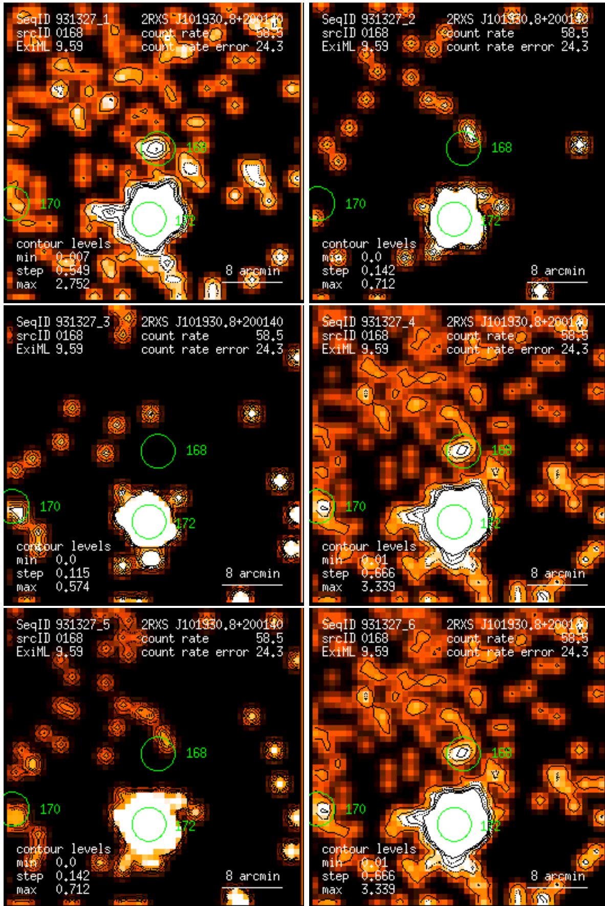
Figure 168: RASS 931327: detection 0168: band rate images, Gaussian filter: (1) PSPC channels 11 – 41, (2) 52 – 90, (3) 91 – 201, (4) 11 – 235, (5) 52 – 201, (6) 11 – 201. Broad band rates in counts/ks. Band rate contour levels in counts/ks/arcmin 2 .
