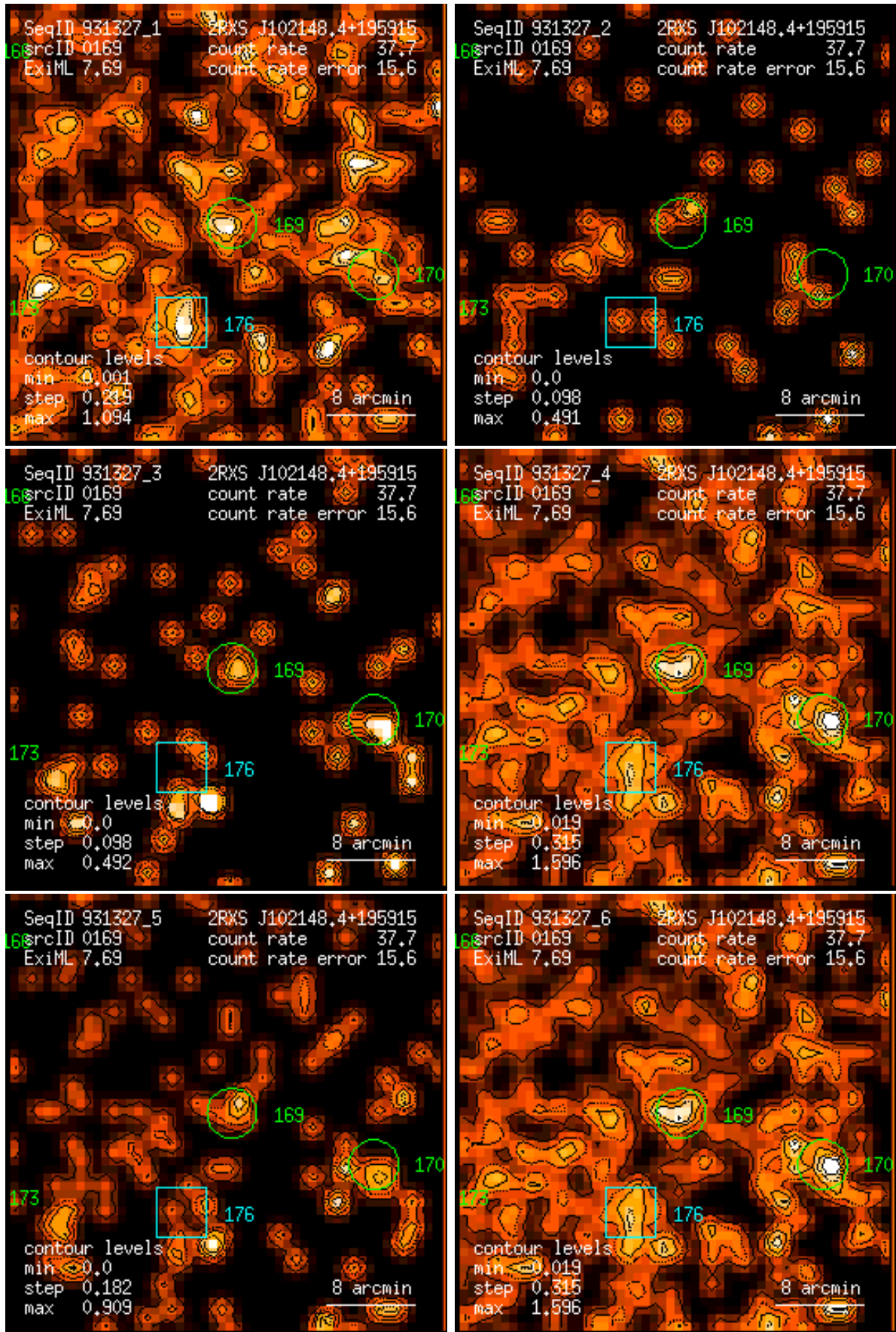
Figure 169: RASS 931327: detection 0169: band rate images, Gaussian filter: (1) PSPC channels 11 – 41, (2) 52 – 90, (3) 91 – 201, (4) 11 – 235, (5) 52 – 201, (6) 11 – 201. Broad band rates in counts/ks. Band rate contour levels in counts/ks/arcmin 2 .
