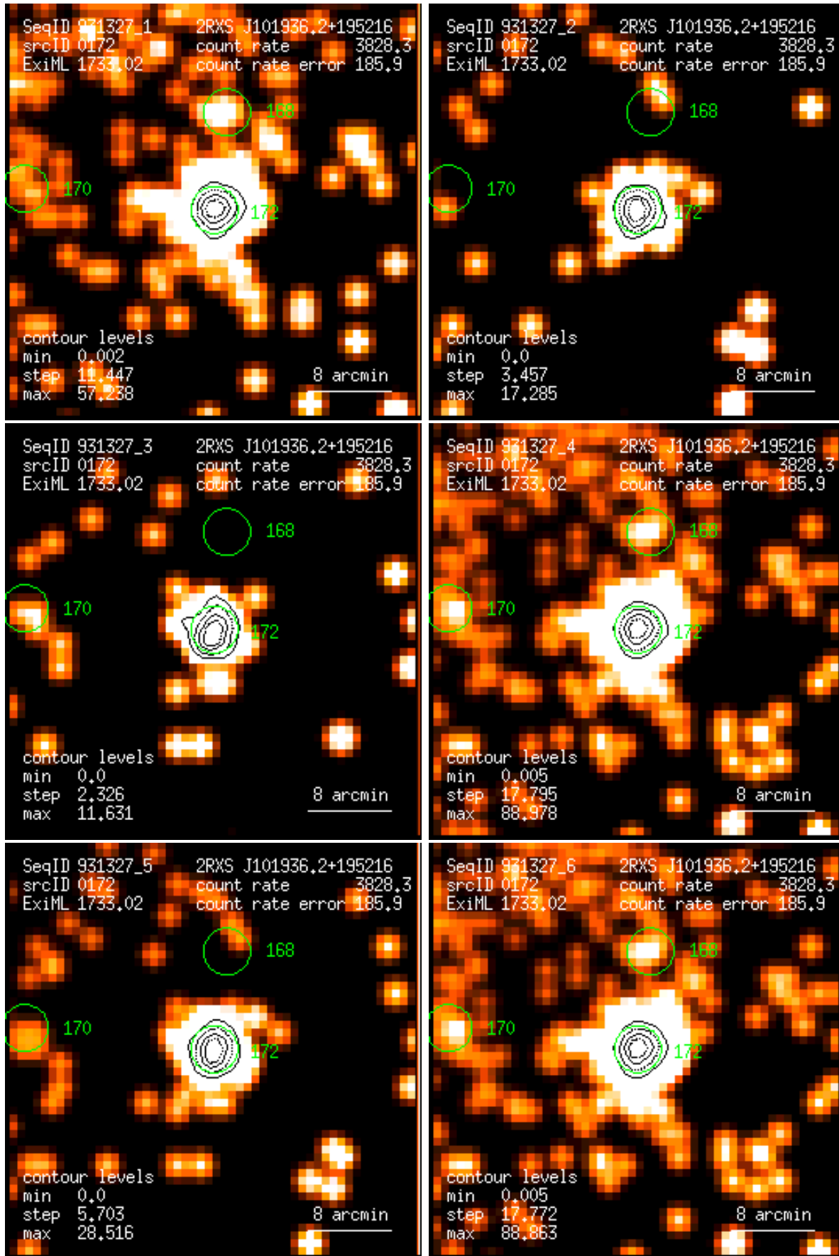
Figure 172: RASS 931327: detection 0172: band rate images, Gaussian filter: (1) PSPC channels 11 – 41, (2) 52 – 90, (3) 91 – 201, (4) 11 – 235, (5) 52 – 201, (6) 11 – 201. Broad band rates in counts/ks. Band rate contour levels in counts/ks/arcmin 2 .
