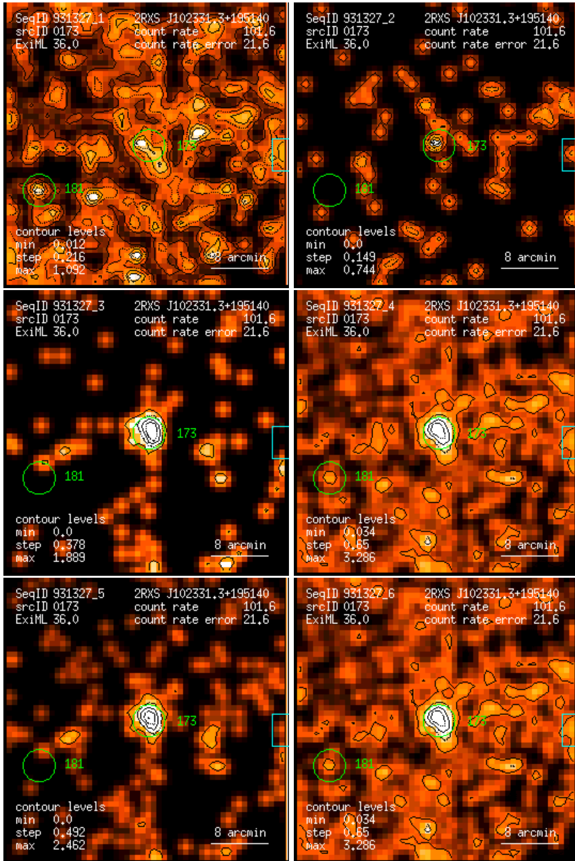
Figure 173: RASS 931327: detection 0173: band rate images, Gaussian filter: (1) PSPC channels 11 – 41, (2) 52 – 90, (3) 91 – 201, (4) 11 – 235, (5) 52 – 201, (6) 11 – 201. Broad band rates in counts/ks. Band rate contour levels in counts/ks/arcmin 2 .
