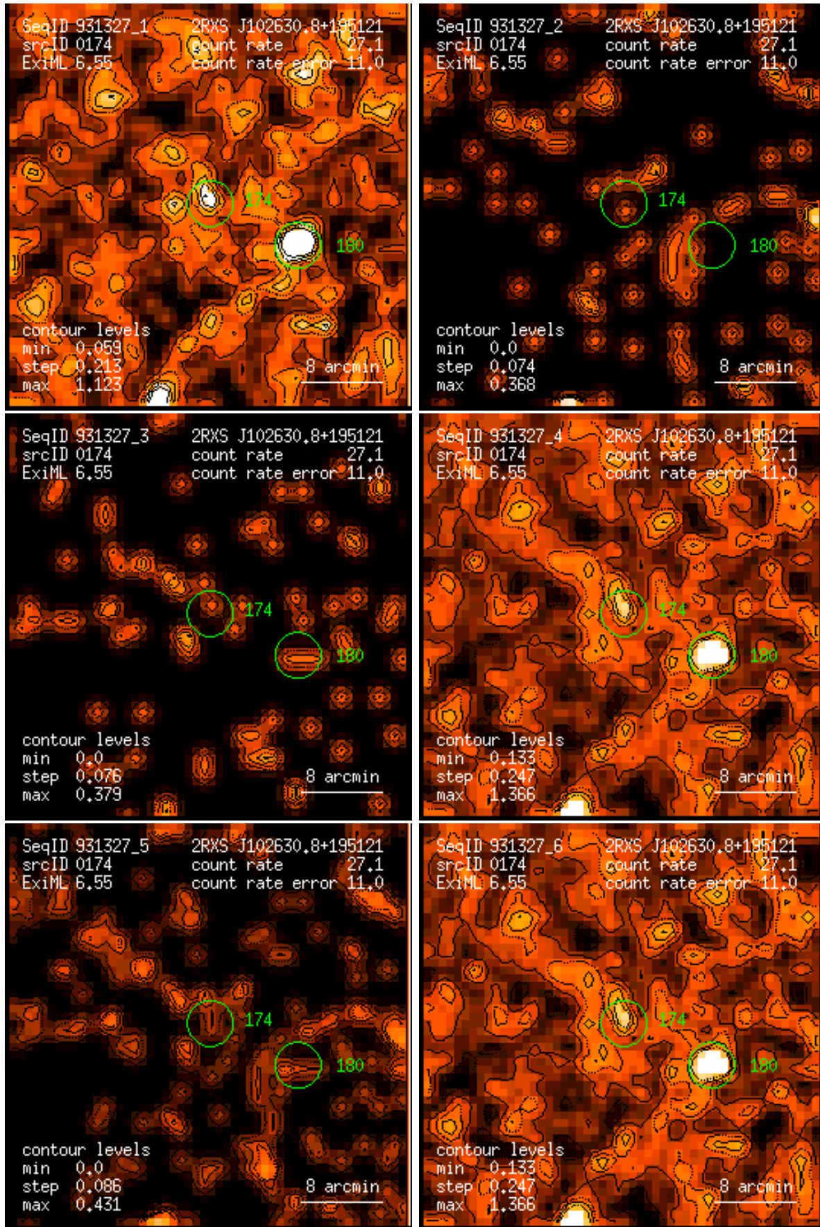
Figure 174: RASS 931327: detection 0174: band rate images, Gaussian filter: (1) PSPC channels 11 – 41, (2) 52 – 90, (3) 91 – 201, (4) 11 – 235, (5) 52 – 201, (6) 11 – 201. Broad band rates in counts/ks. Band rate contour levels in counts/ks/arcmin 2 .
