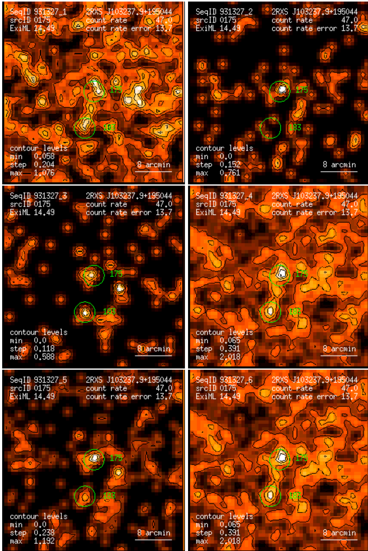
Figure 175: RASS 931327: detection 0175: band rate images, Gaussian filter: (1) PSPC channels 11 – 41, (2) 52 – 90, (3) 91 – 201, (4) 11 – 235, (5) 52 – 201, (6) 11 – 201. Broad band rates in counts/ks. Band rate contour levels in counts/ks/arcmin 2 .
