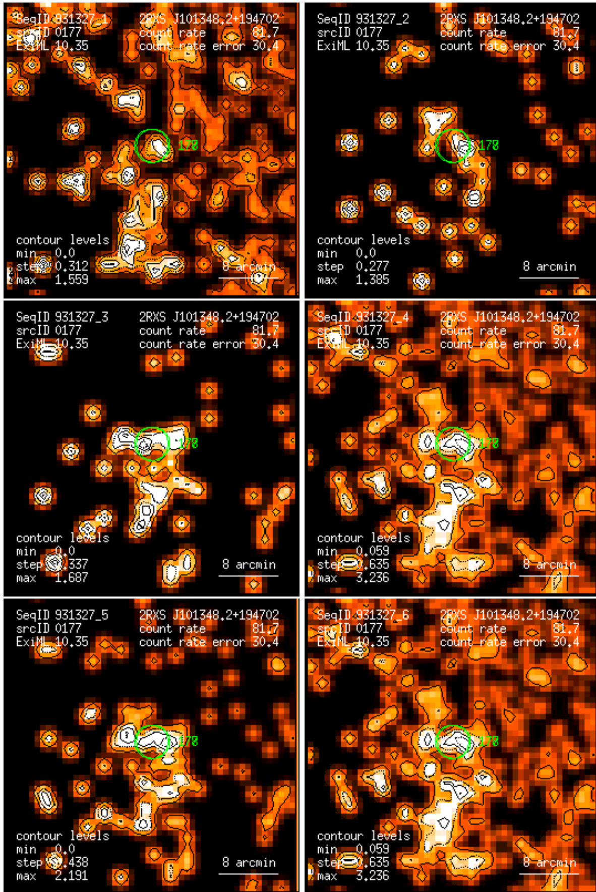
Figure 177: RASS 931327: detection 0177: band rate images, Gaussian filter: (1) PSPC channels 11 – 41, (2) 52 – 90, (3) 91 – 201, (4) 11 – 235, (5) 52 – 201, (6) 11 – 201. Broad band rates in counts/ks. Band rate contour levels in counts/ks/arcmin 2 .
