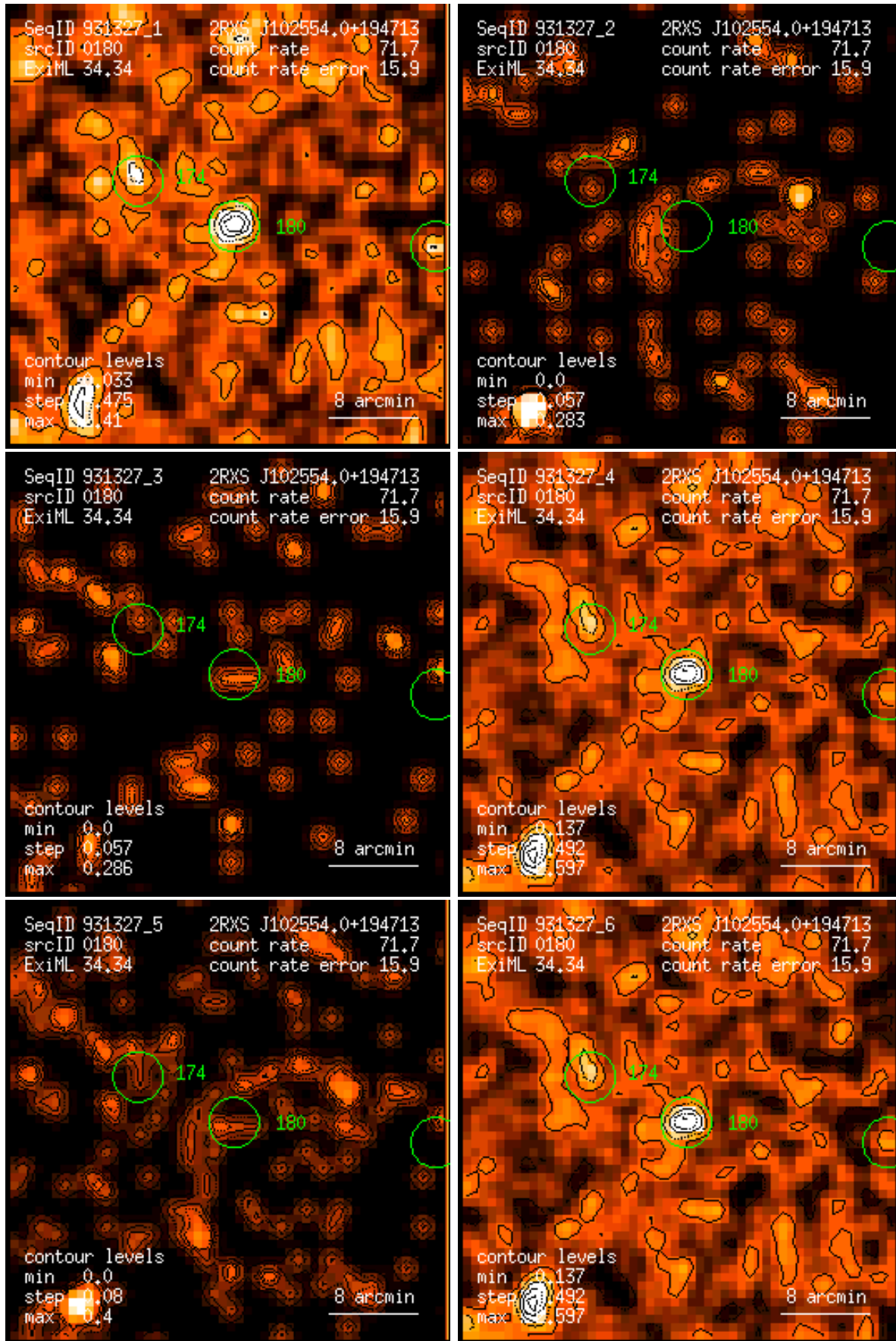
Figure 180: RASS 931327: detection 0180: band rate images, Gaussian filter: (1) PSPC channels 11 – 41, (2) 52 – 90, (3) 91 – 201, (4) 11 – 235, (5) 52 – 201, (6) 11 – 201. Broad band rates in counts/ks. Band rate contour levels in counts/ks/arcmin 2 .
