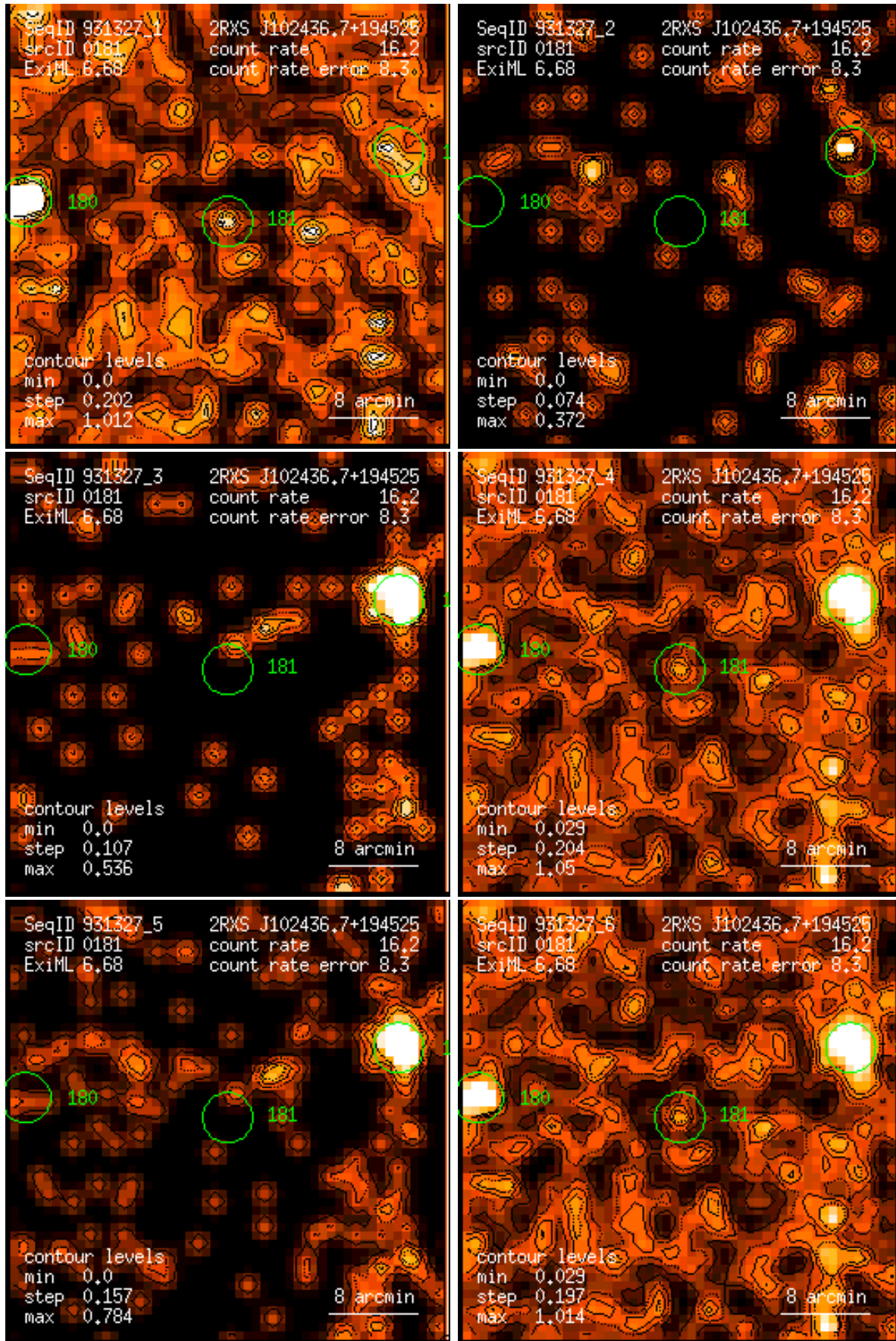
Figure 181: RASS 931327: detection 0181: band rate images, Gaussian filter: (1) PSPC channels 11 – 41, (2) 52 – 90, (3) 91 – 201, (4) 11 – 235, (5) 52 – 201, (6) 11 – 201. Broad band rates in counts/ks. Band rate contour levels in counts/ks/arcmin 2 .
