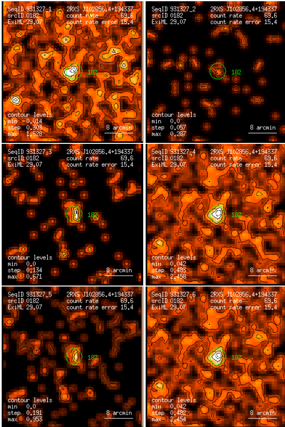
Figure 182: RASS 931327: detection 0182: band rate images, Gaussian filter: (1) PSPC channels 11 – 41, (2) 52 – 90, (3) 91 – 201, (4) 11 – 235, (5) 52 – 201, (6) 11 – 201. Broad band rates in counts/ks. Band rate contour levels in counts/ks/arcmin 2 .
