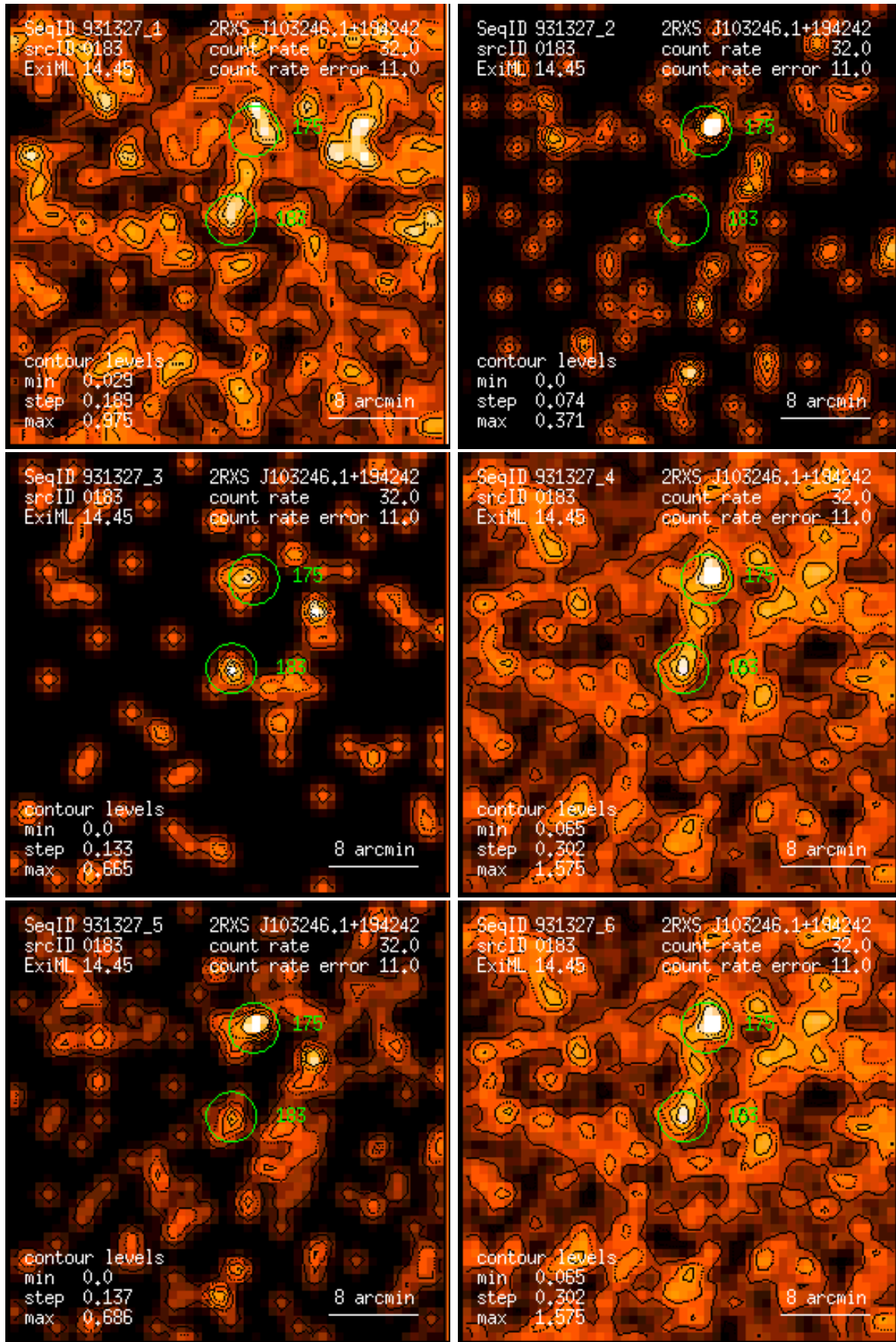
Figure 183: RASS 931327: detection 0183: band rate images, Gaussian filter: (1) PSPC channels 11 – 41, (2) 52 – 90, (3) 91 – 201, (4) 11 – 235, (5) 52 – 201, (6) 11 – 201. Broad band rates in counts/ks. Band rate contour levels in counts/ks/arcmin 2 .
