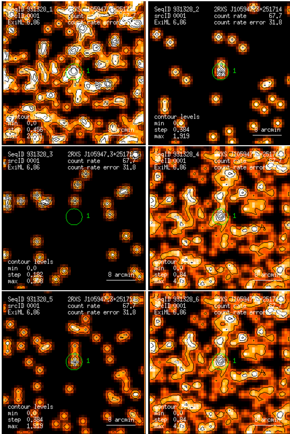
Figure 1: RASS 931328: detection 0001: band rate images, Gaussian filter: (1) PSPC channels 11 – 41, (2) 52 – 90, (3) 91 – 201, (4) 11 – 235, (5) 52 – 201, (6) 11 – 201. Broad band rates in counts/ks. Band rate contour levels in counts/ks/arcmin 2 .
