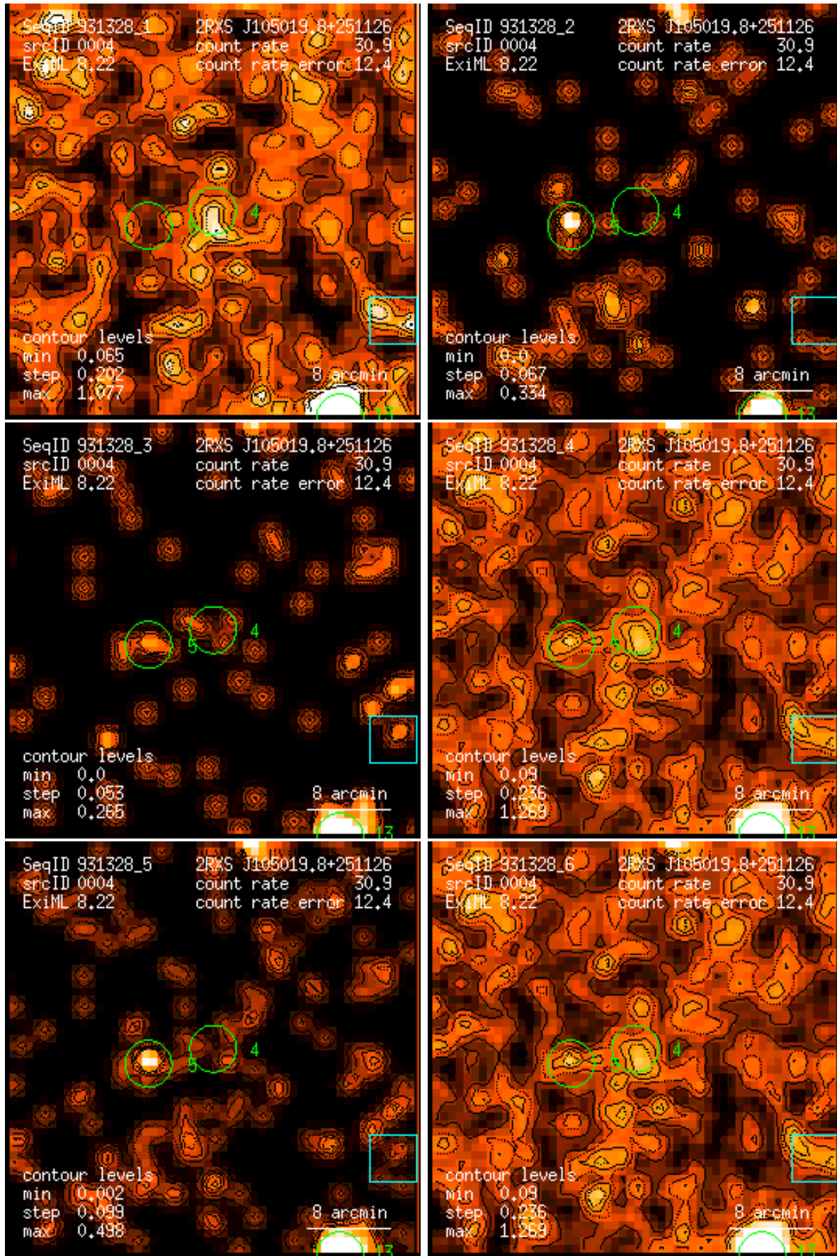
Figure 4: RASS 931328: detection 0004: band rate images, Gaussian filter: (1) PSPC channels 11 – 41, (2) 52 – 90, (3) 91 – 201, (4) 11 – 235, (5) 52 – 201, (6) 11 – 201. Broad band rates in counts/ks. Band rate contour levels in counts/ks/arcmin 2 .
