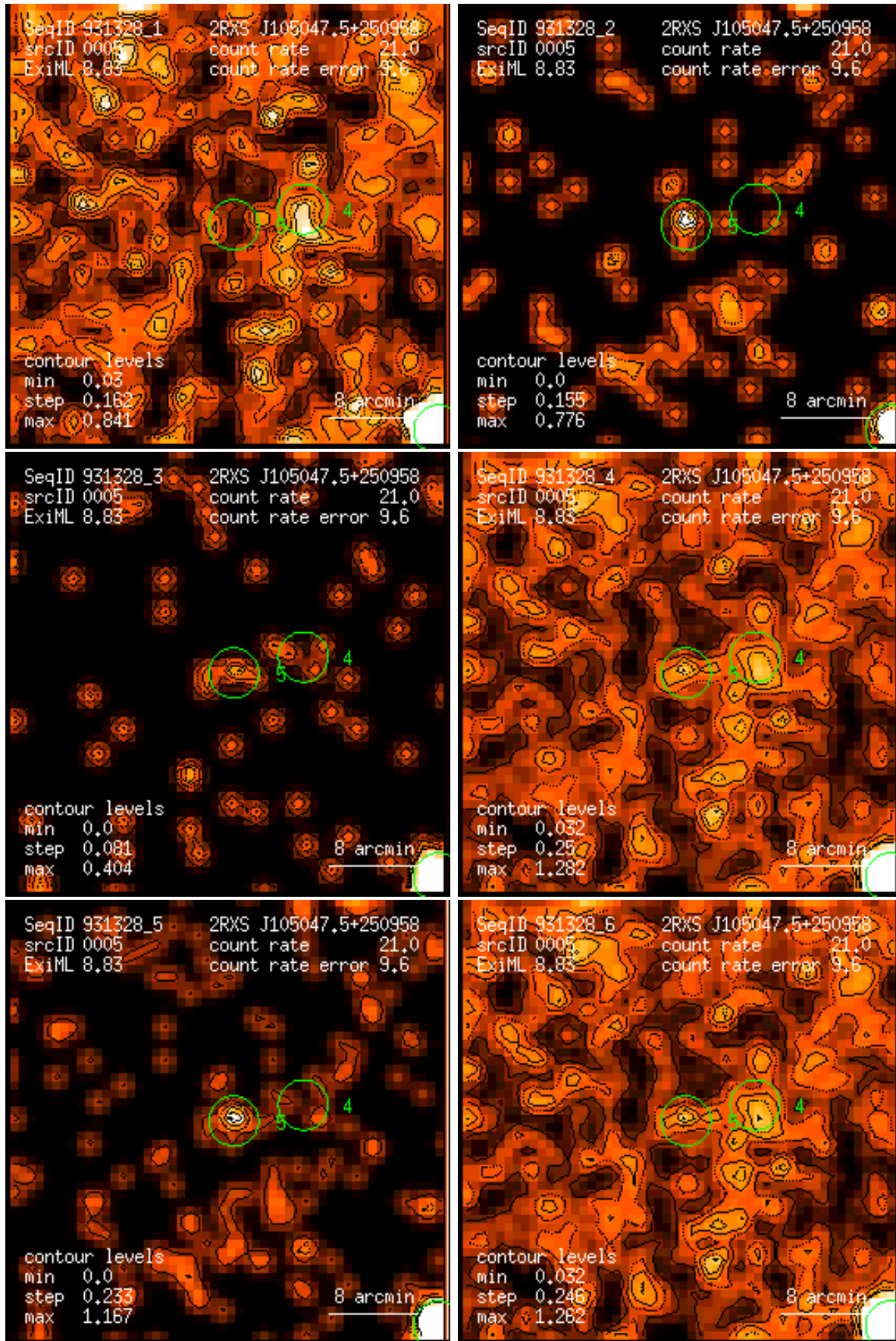
Figure 5: RASS 931328: detection 0005: band rate images, Gaussian filter: (1) PSPC channels 11 – 41, (2) 52 – 90, (3) 91 – 201, (4) 11 – 235, (5) 52 – 201, (6) 11 – 201. Broad band rates in counts/ks. Band rate contour levels in counts/ks/arcmin 2 .
