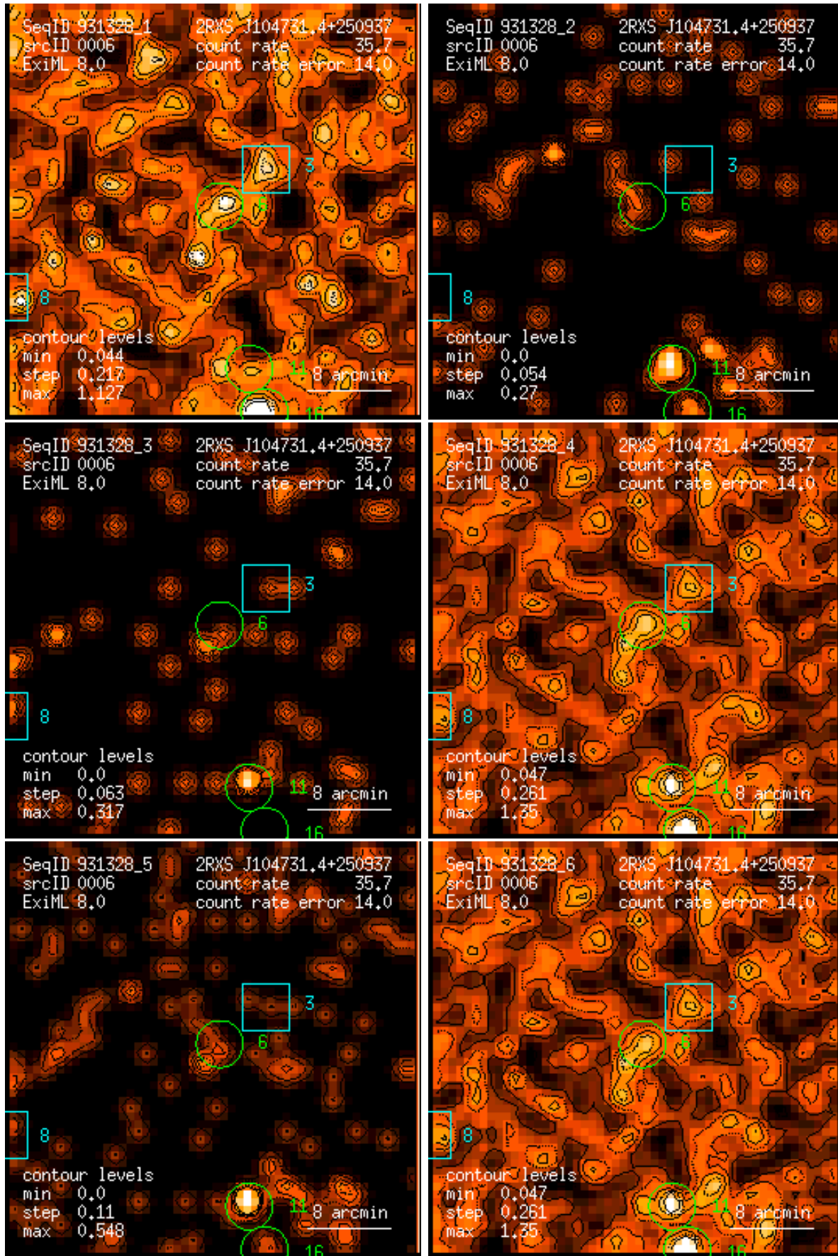
Figure 6: RASS 931328: detection 0006: band rate images, Gaussian filter: (1) PSPC channels 11 – 41, (2) 52 – 90, (3) 91 – 201, (4) 11 – 235, (5) 52 – 201, (6) 11 – 201. Broad band rates in counts/ks. Band rate contour levels in counts/ks/arcmin 2 .
