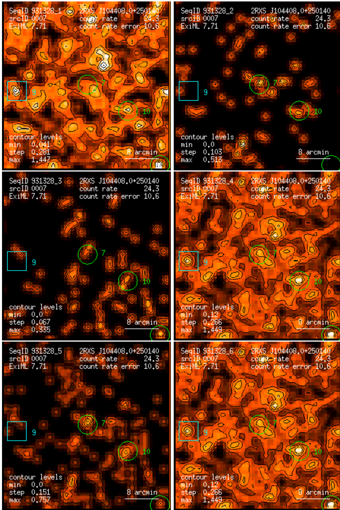
Figure 7: RASS 931328: detection 0007: band rate images, Gaussian filter: (1) PSPC channels 11 – 41, (2) 52 – 90, (3) 91 – 201, (4) 11 – 235, (5) 52 – 201, (6) 11 – 201. Broad band rates in counts/ks. Band rate contour levels in counts/ks/arcmin 2 .
