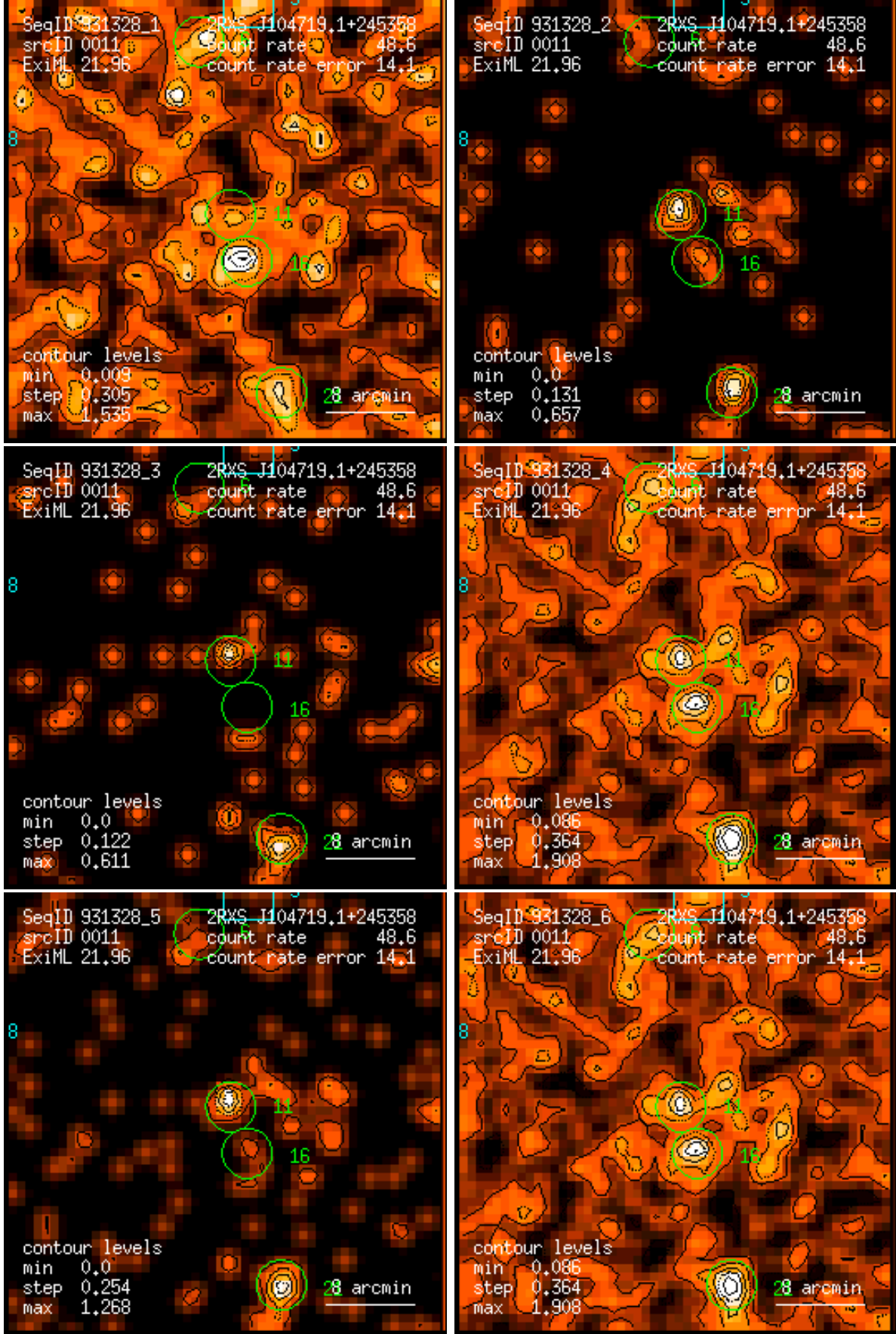
Figure 11: RASS 931328: detection 0011: band rate images, Gaussian filter: (1) PSPC channels 11 – 41, (2) 52 – 90, (3) 91 – 201, (4) 11 – 235, (5) 52 – 201, (6) 11 – 201. Broad band rates in counts/ks. Band rate contour levels in counts/ks/arcmin 2 .
