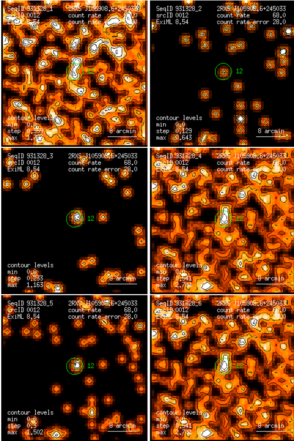
Figure 12: RASS 931328: detection 0012: band rate images, Gaussian filter: (1) PSPC channels 11 – 41, (2) 52 – 90, (3) 91 – 201, (4) 11 – 235, (5) 52 – 201, (6) 11 – 201. Broad band rates in counts/ks. Band rate contour levels in counts/ks/arcmin 2 .
