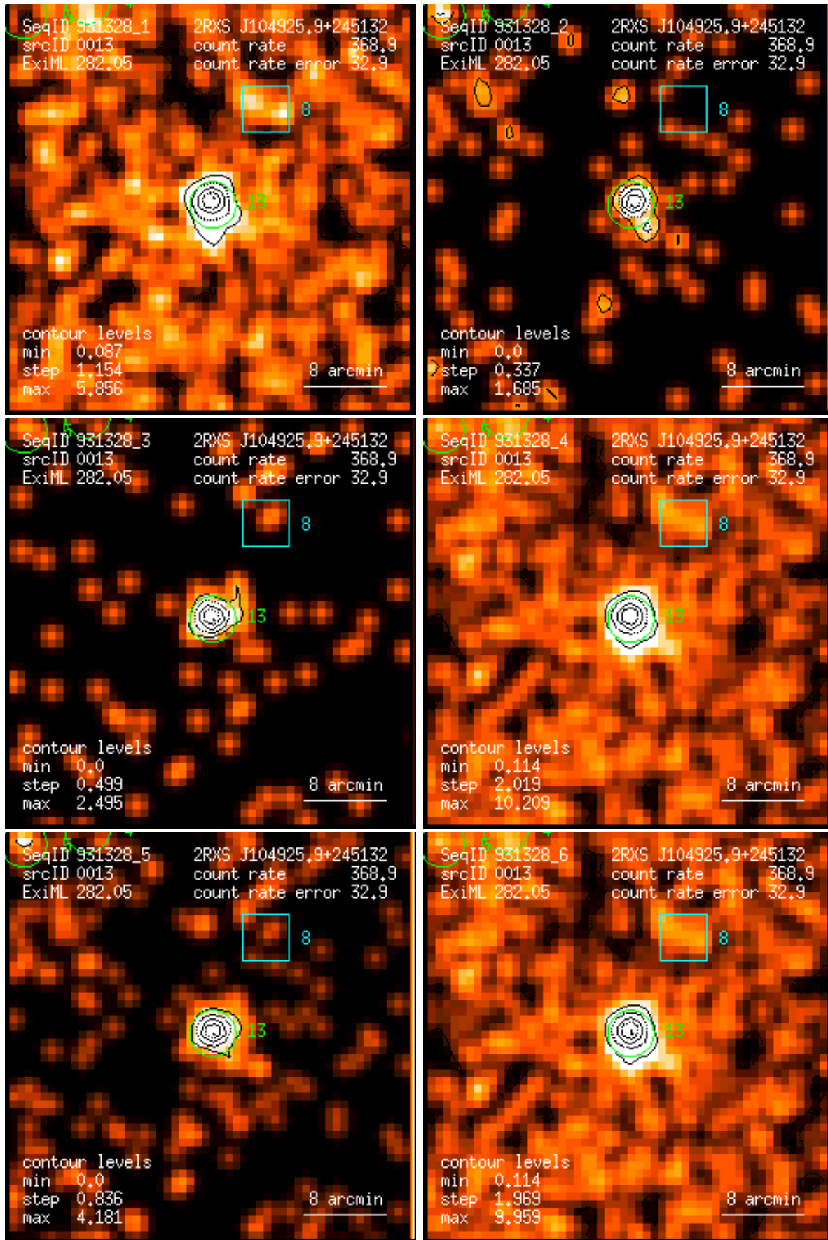
Figure 13: RASS 931328: detection 0013: band rate images, Gaussian filter: (1) PSPC channels 11 – 41, (2) 52 – 90, (3) 91 – 201, (4) 11 – 235, (5) 52 – 201, (6) 11 – 201. Broad band rates in counts/ks. Band rate contour levels in counts/ks/arcmin 2 .
