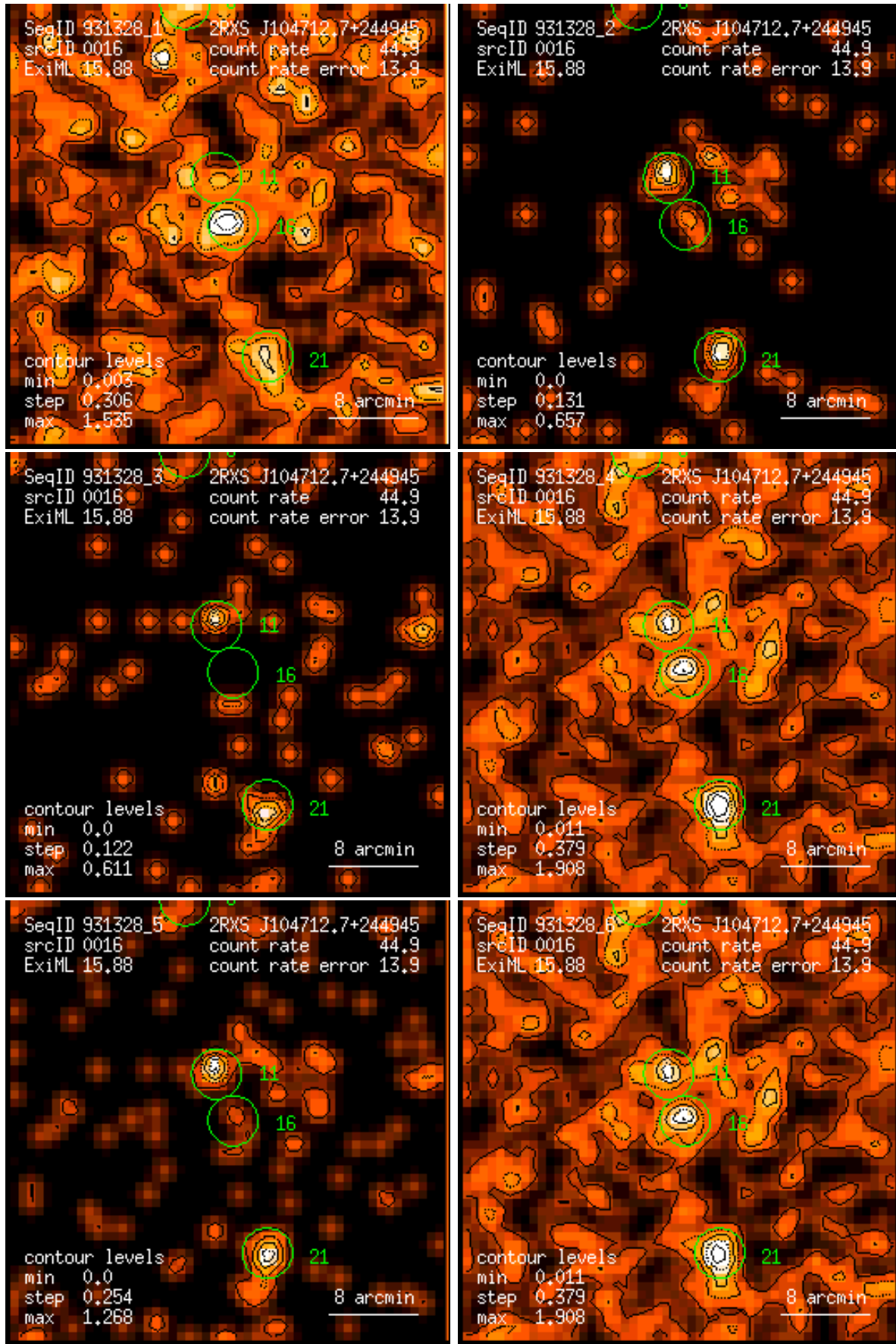
Figure 16: RASS 931328: detection 0016: band rate images, Gaussian filter: (1) PSPC channels 11 – 41, (2) 52 – 90, (3) 91 – 201, (4) 11 – 235, (5) 52 – 201, (6) 11 – 201. Broad band rates in counts/ks. Band rate contour levels in counts/ks/arcmin 2 .
