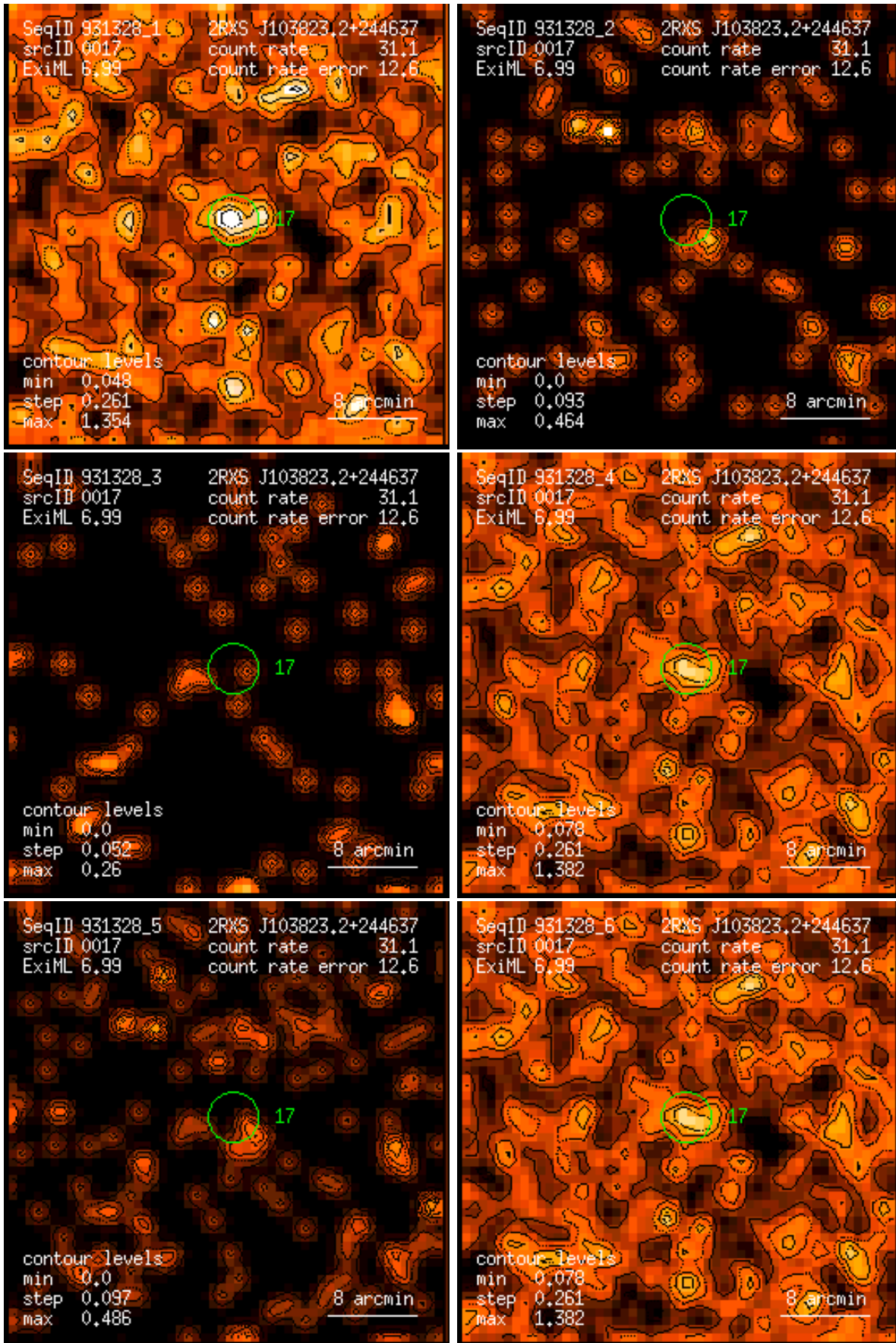
Figure 17: RASS 931328: detection 0017: band rate images, Gaussian filter: (1) PSPC channels 11 – 41, (2) 52 – 90, (3) 91 – 201, (4) 11 – 235, (5) 52 – 201, (6) 11 – 201. Broad band rates in counts/ks. Band rate contour levels in counts/ks/arcmin 2 .
