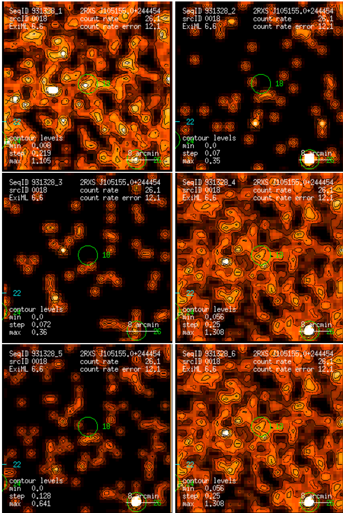
Figure 18: RASS 931328: detection 0018: band rate images, Gaussian filter: (1) PSPC channels 11 – 41, (2) 52 – 90, (3) 91 – 201, (4) 11 – 235, (5) 52 – 201, (6) 11 – 201. Broad band rates in counts/ks. Band rate contour levels in counts/ks/arcmin 2 .
