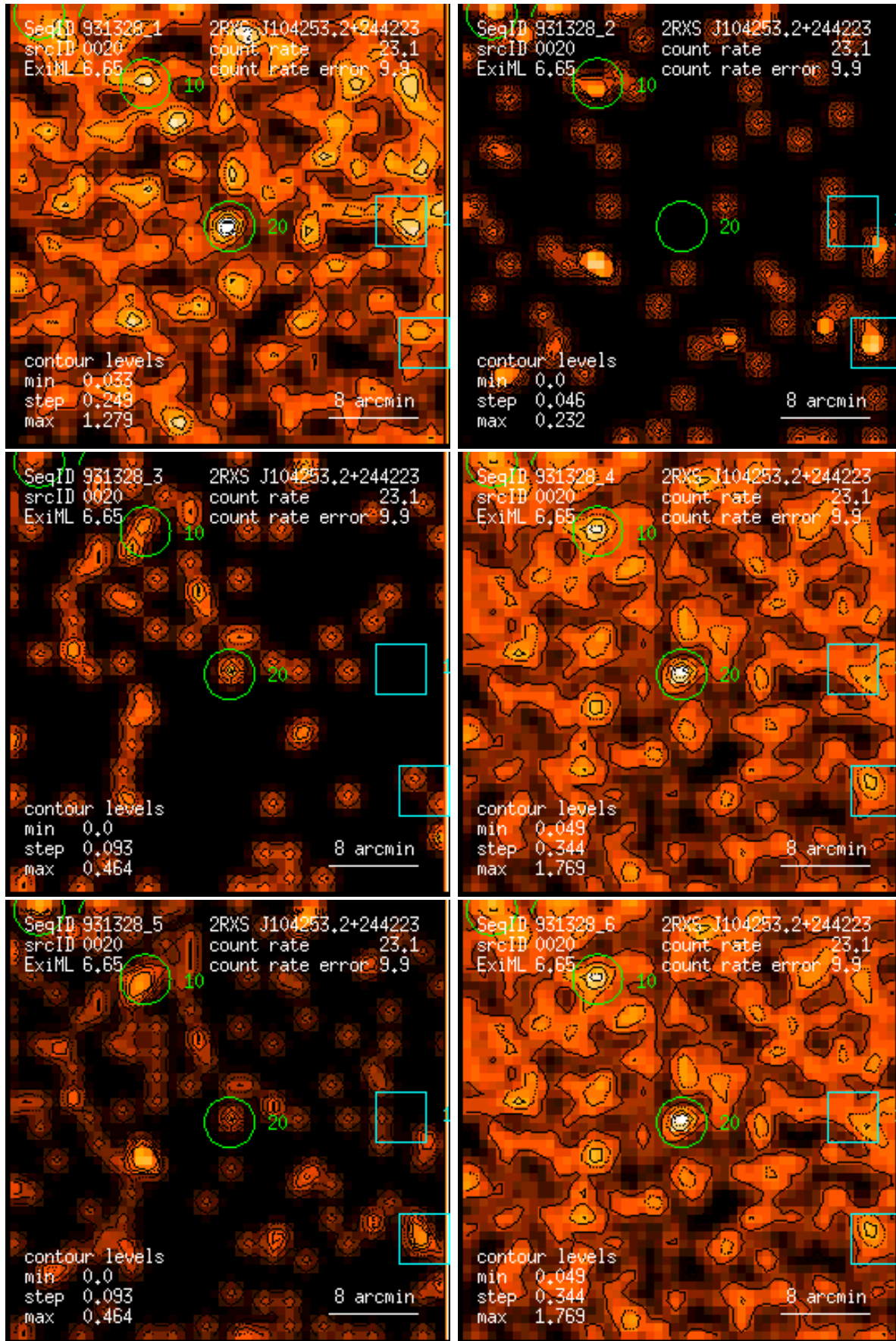
Figure 20: RASS 931328: detection 0020: band rate images, Gaussian filter: (1) PSPC channels 11 – 41, (2) 52 – 90, (3) 91 – 201, (4) 11 – 235, (5) 52 – 201, (6) 11 – 201. Broad band rates in counts/ks. Band rate contour levels in counts/ks/arcmin 2 .
