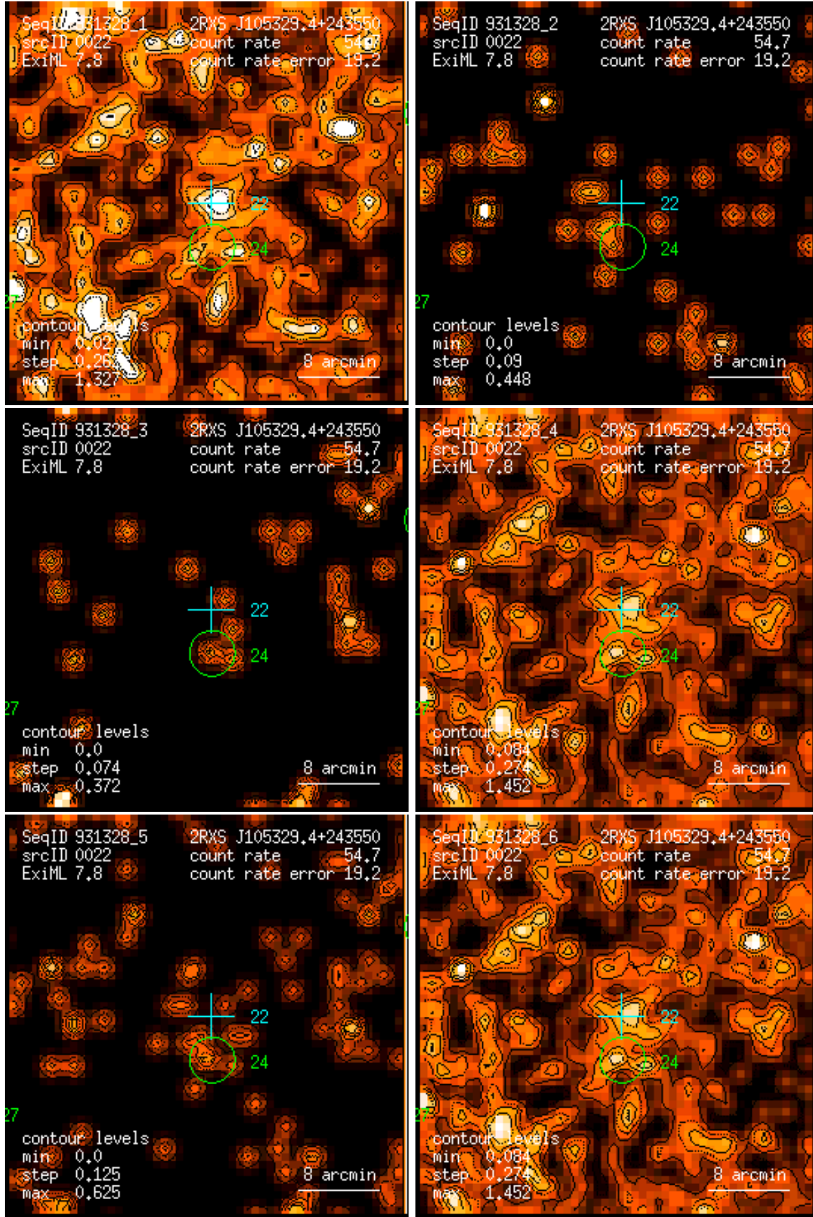
Figure 22: RASS 931328: detection 0022: band rate images, Gaussian filter: (1) PSPC channels 11 – 41, (2) 52 – 90, (3) 91 – 201, (4) 11 – 235, (5) 52 – 201, (6) 11 – 201. Broad band rates in counts/ks. Band rate contour levels in counts/ks/arcmin 2 .
