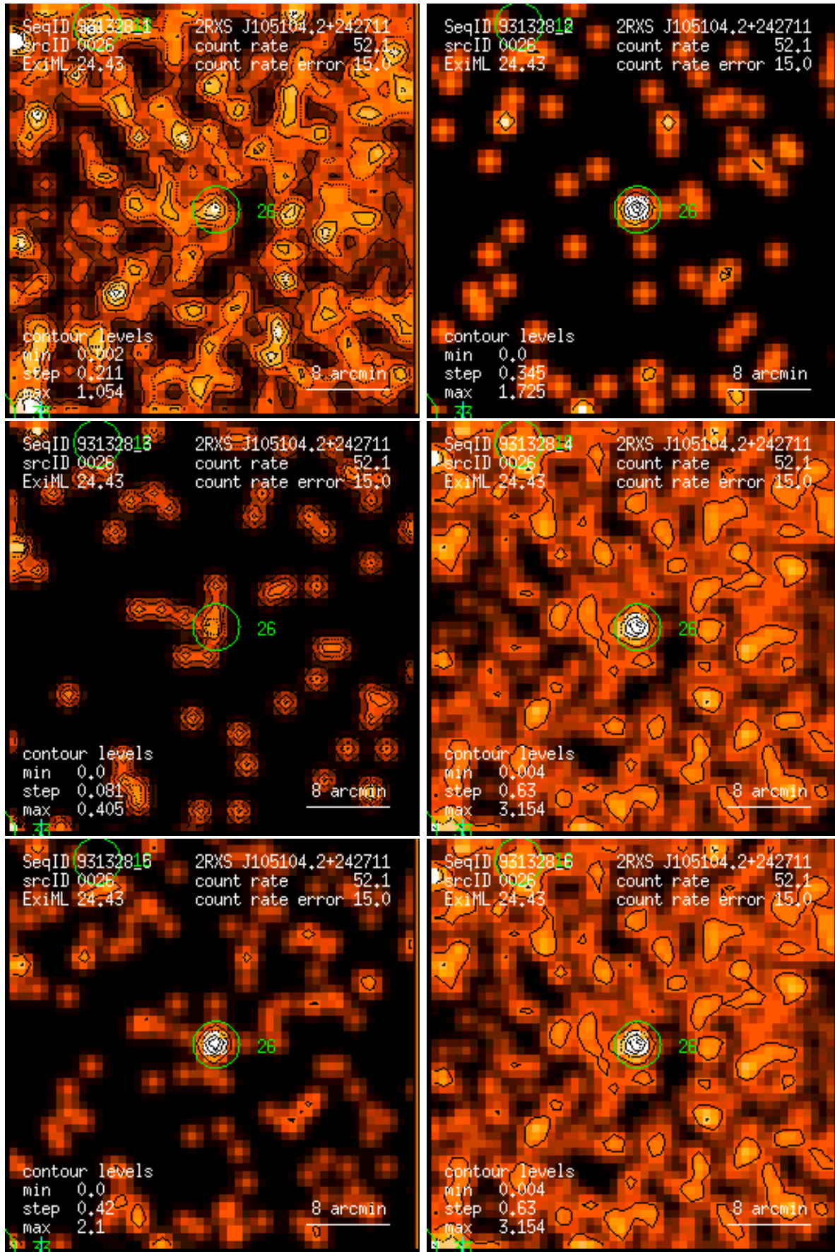
Figure 26: RASS 931328: detection 0026: band rate images, Gaussian filter: (1) PSPC channels 11 – 41, (2) 52 – 90, (3) 91 – 201, (4) 11 – 235, (5) 52 – 201, (6) 11 – 201. Broad band rates in counts/ks. Band rate contour levels in counts/ks/arcmin 2 .
