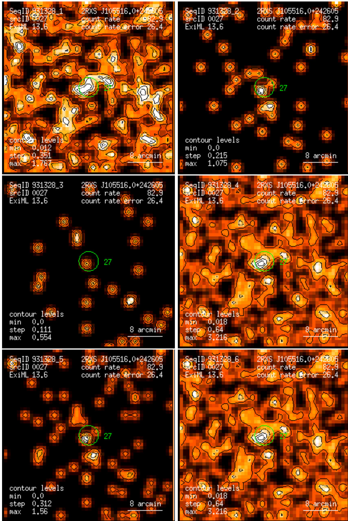
Figure 27: RASS 931328: detection 0027: band rate images, Gaussian filter: (1) PSPC channels 11 – 41, (2) 52 – 90, (3) 91 – 201, (4) 11 – 235, (5) 52 – 201, (6) 11 – 201. Broad band rates in counts/ks. Band rate contour levels in counts/ks/arcmin 2 .
