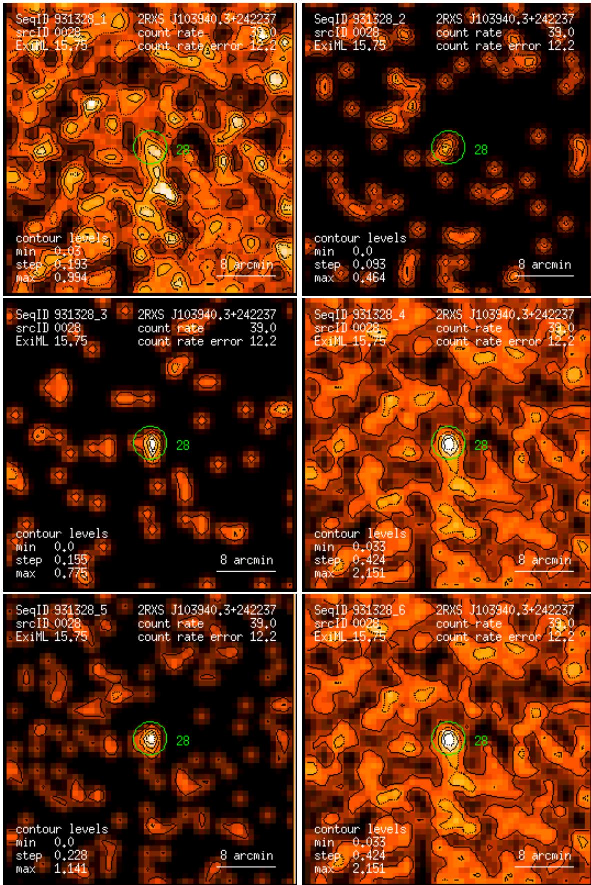
Figure 28: RASS 931328: detection 0028: band rate images, Gaussian filter: (1) PSPC channels 11 – 41, (2) 52 – 90, (3) 91 – 201, (4) 11 – 235, (5) 52 – 201, (6) 11 – 201. Broad band rates in counts/ks. Band rate contour levels in counts/ks/arcmin 2 .
