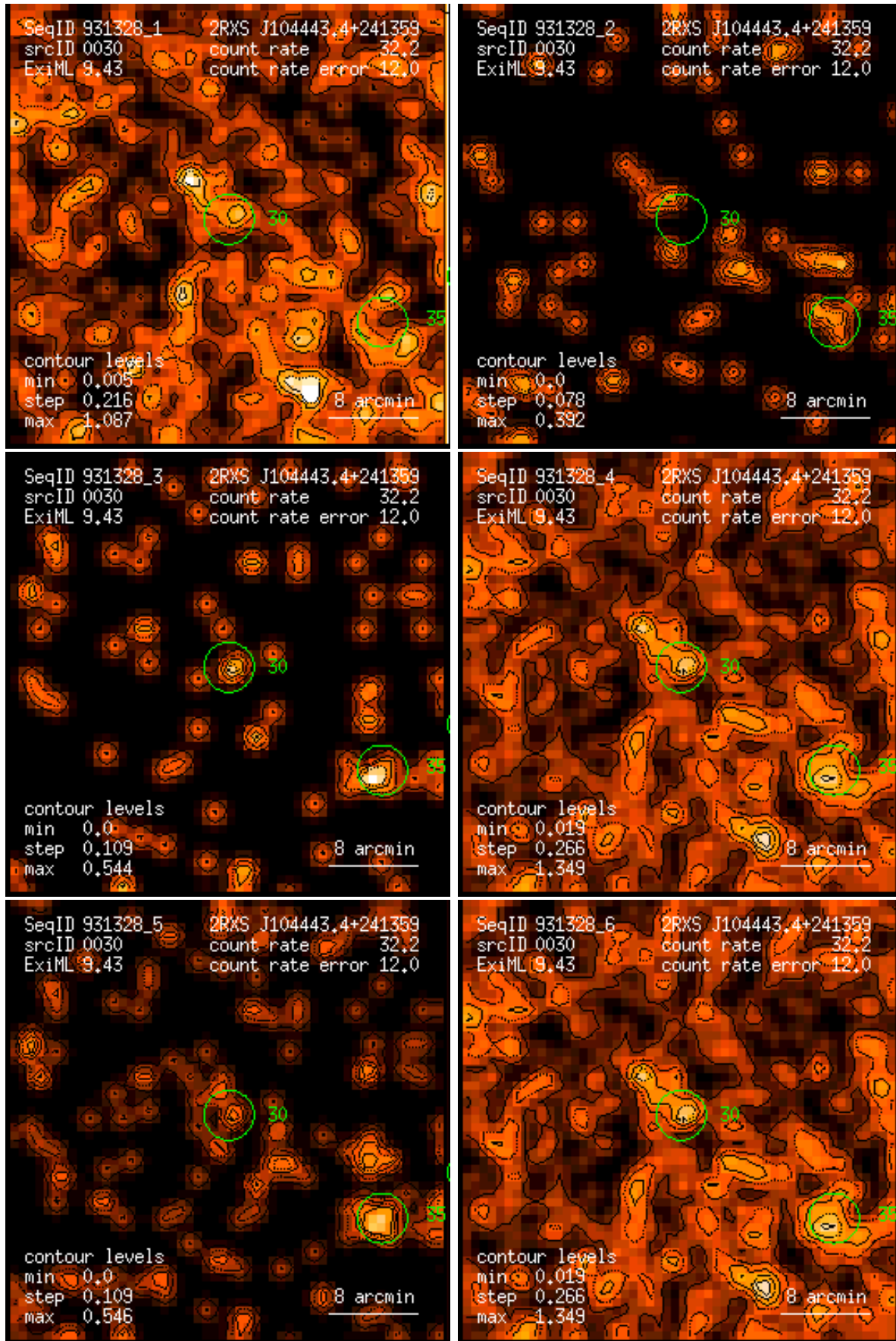
Figure 30: RASS 931328: detection 0030: band rate images, Gaussian filter: (1) PSPC channels 11 – 41, (2) 52 – 90, (3) 91 – 201, (4) 11 – 235, (5) 52 – 201, (6) 11 – 201. Broad band rates in counts/ks. Band rate contour levels in counts/ks/arcmin 2 .
