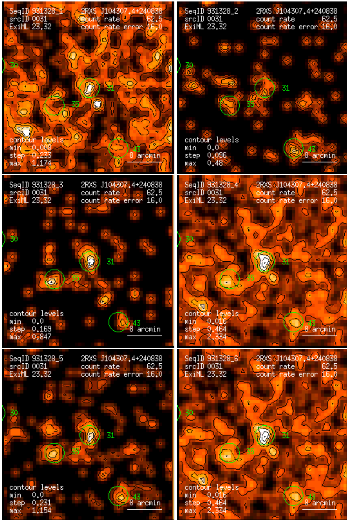
Figure 31: RASS 931328: detection 0031: band rate images, Gaussian filter: (1) PSPC channels 11 – 41, (2) 52 – 90, (3) 91 – 201, (4) 11 – 235, (5) 52 – 201, (6) 11 – 201. Broad band rates in counts/ks. Band rate contour levels in counts/ks/arcmin 2 .
