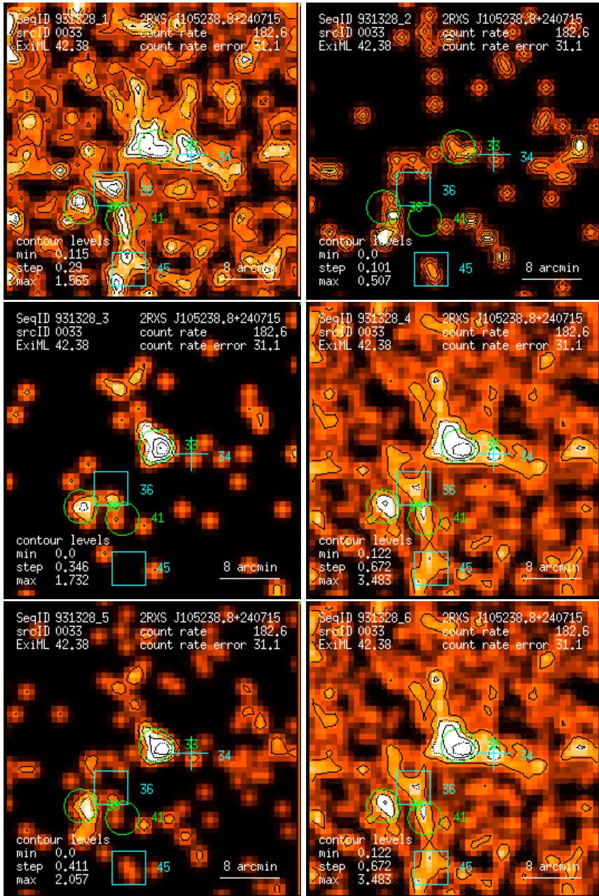
Figure 33: RASS 931328: detection 0033: band rate images, Gaussian filter: (1) PSPC channels 11 – 41, (2) 52 – 90, (3) 91 – 201, (4) 11 – 235, (5) 52 – 201, (6) 11 – 201. Broad band rates in counts/ks. Band rate contour levels in counts/ks/arcmin 2 .
