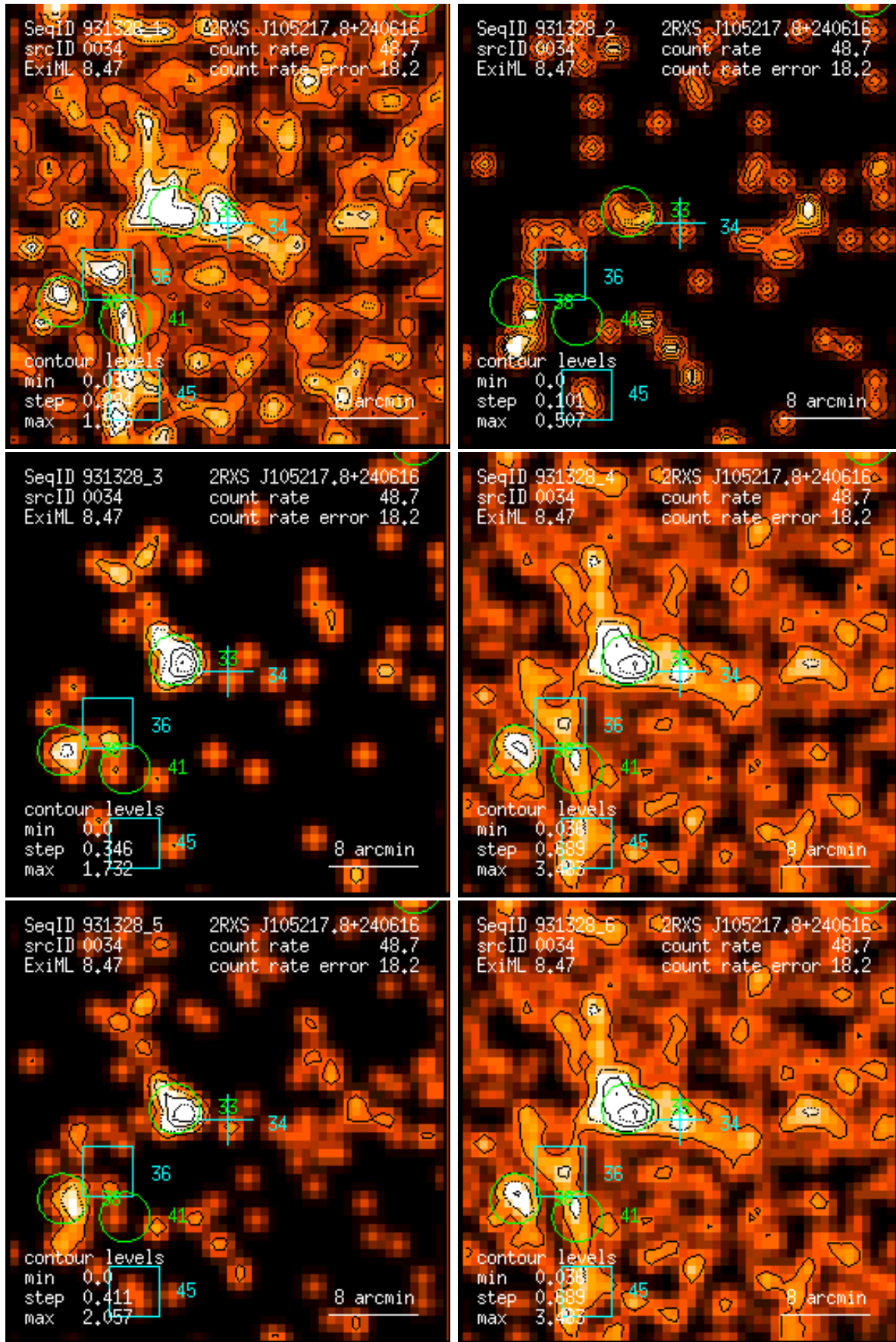
Figure 34: RASS 931328: detection 0034: band rate images, Gaussian filter: (1) PSPC channels 11 – 41, (2) 52 – 90, (3) 91 – 201, (4) 11 – 235, (5) 52 – 201, (6) 11 – 201. Broad band rates in counts/ks. Band rate contour levels in counts/ks/arcmin 2 .
