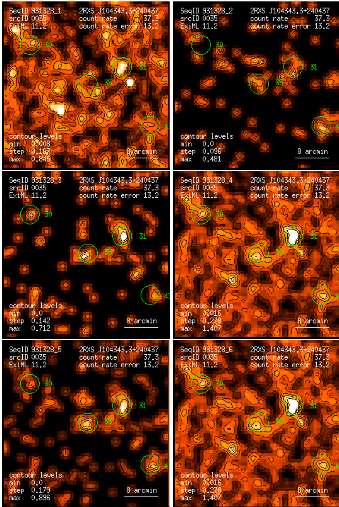
Figure 35: RASS 931328: detection 0035: band rate images, Gaussian filter: (1) PSPC channels 11 – 41, (2) 52 – 90, (3) 91 – 201, (4) 11 – 235, (5) 52 – 201, (6) 11 – 201. Broad band rates in counts/ks. Band rate contour levels in counts/ks/arcmin 2 .
