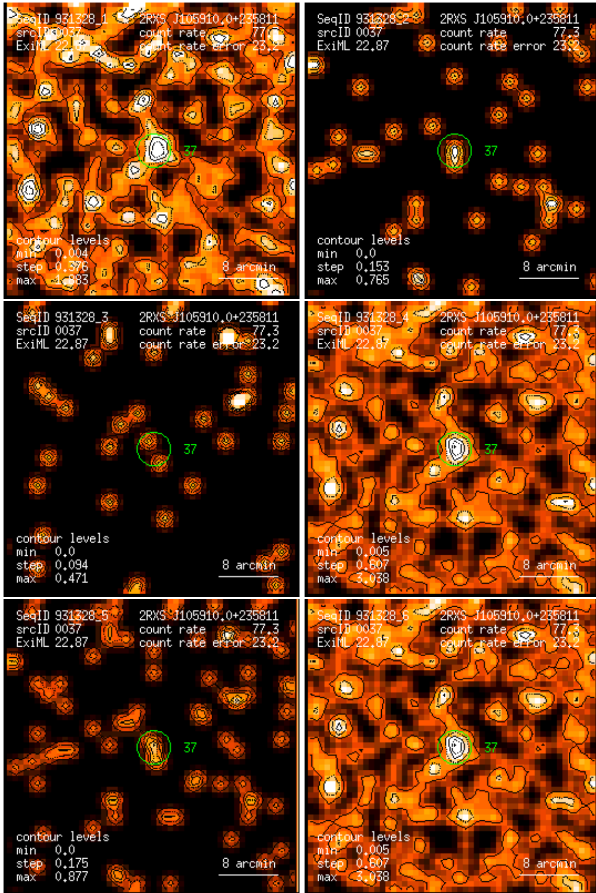
Figure 37: RASS 931328: detection 0037: band rate images, Gaussian filter: (1) PSPC channels 11 – 41, (2) 52 – 90, (3) 91 – 201, (4) 11 – 235, (5) 52 – 201, (6) 11 – 201. Broad band rates in counts/ks. Band rate contour levels in counts/ks/arcmin 2 .
