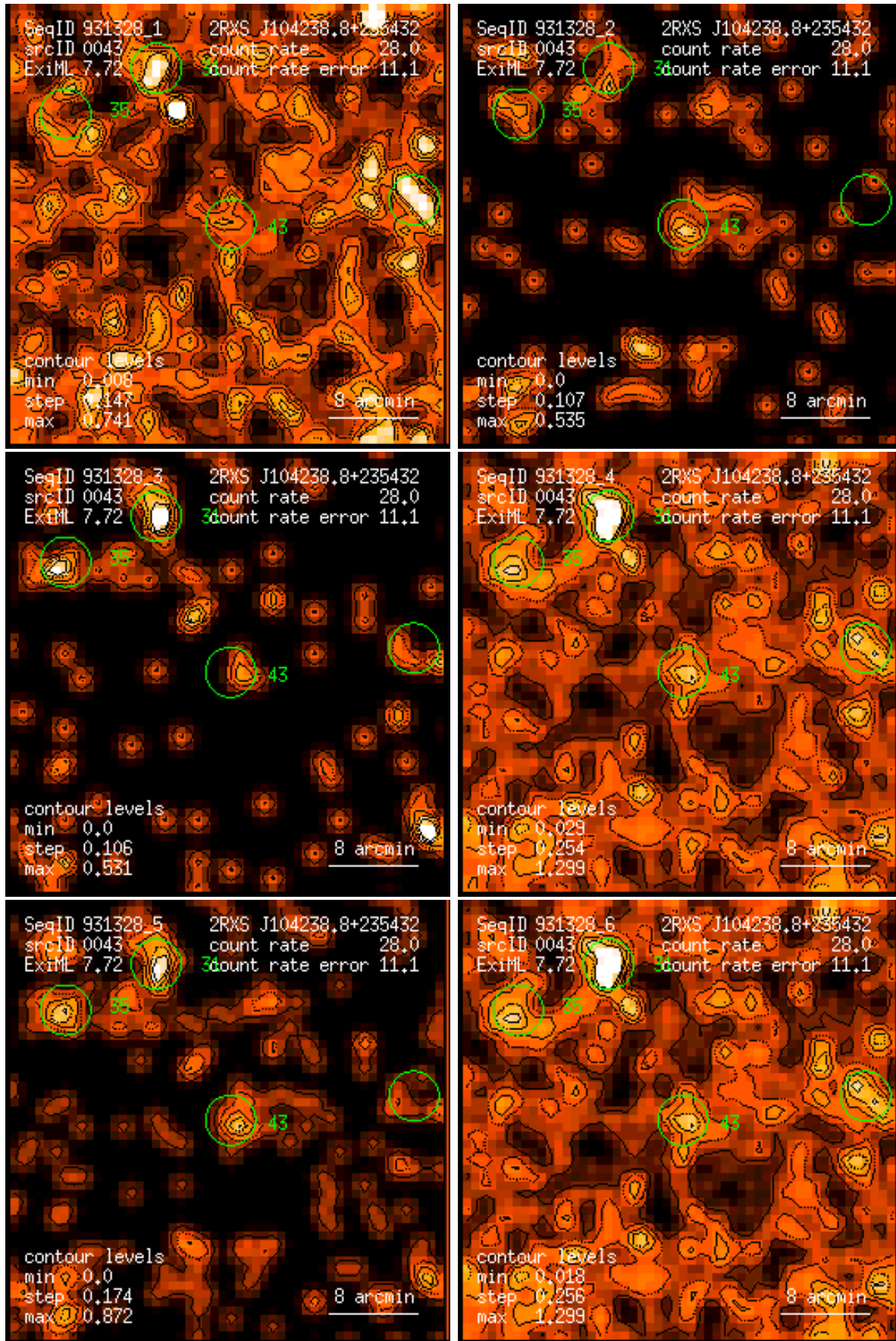
Figure 43: RASS 931328: detection 0043: band rate images, Gaussian filter: (1) PSPC channels 11 – 41, (2) 52 – 90, (3) 91 – 201, (4) 11 – 235, (5) 52 – 201, (6) 11 – 201. Broad band rates in counts/ks. Band rate contour levels in counts/ks/arcmin 2 .
