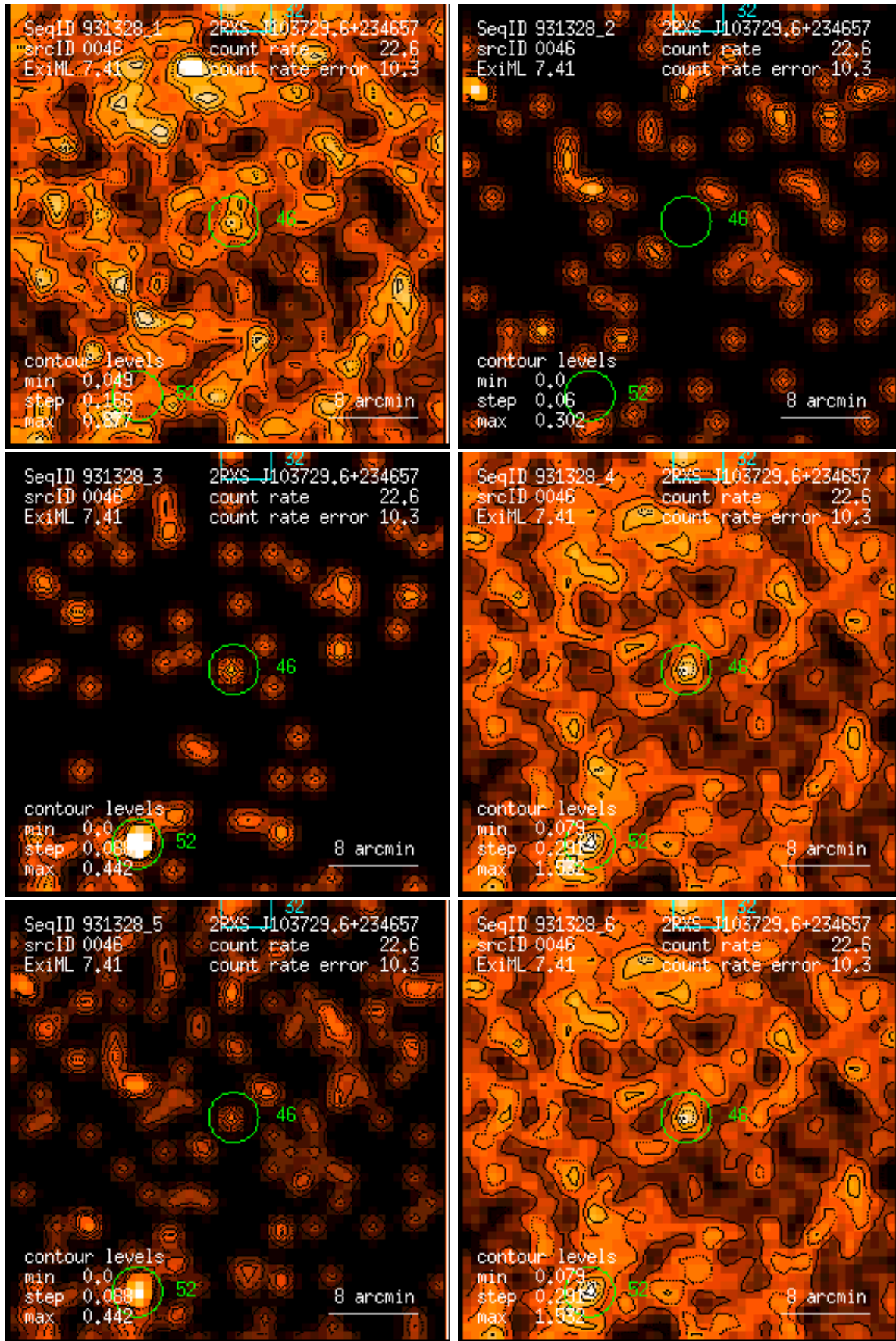
Figure 46: RASS 931328: detection 0046: band rate images, Gaussian filter: (1) PSPC channels 11 – 41, (2) 52 – 90, (3) 91 – 201, (4) 11 – 235, (5) 52 – 201, (6) 11 – 201. Broad band rates in counts/ks. Band rate contour levels in counts/ks/arcmin 2 .
