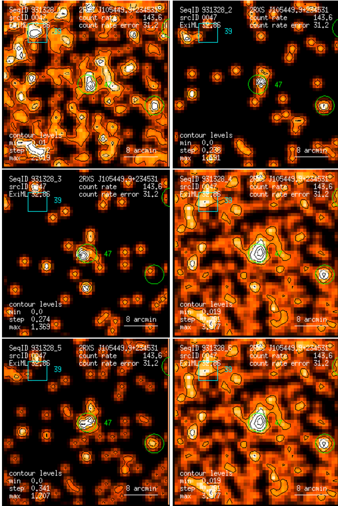
Figure 47: RASS 931328: detection 0047: band rate images, Gaussian filter: (1) PSPC channels 11 – 41, (2) 52 – 90, (3) 91 – 201, (4) 11 – 235, (5) 52 – 201, (6) 11 – 201. Broad band rates in counts/ks. Band rate contour levels in counts/ks/arcmin 2 .
