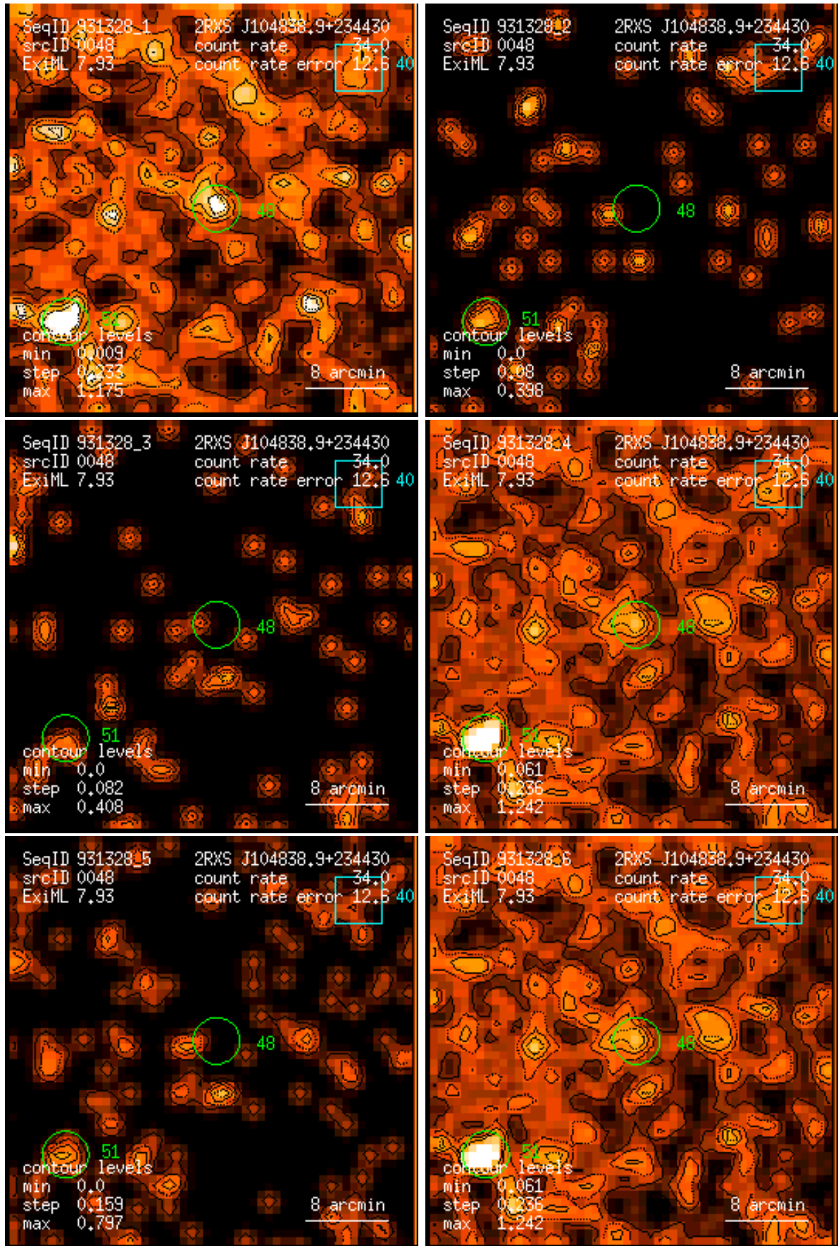
Figure 48: RASS 931328: detection 0048: band rate images, Gaussian filter: (1) PSPC channels 11 – 41, (2) 52 – 90, (3) 91 – 201, (4) 11 – 235, (5) 52 – 201, (6) 11 – 201. Broad band rates in counts/ks. Band rate contour levels in counts/ks/arcmin 2 .
