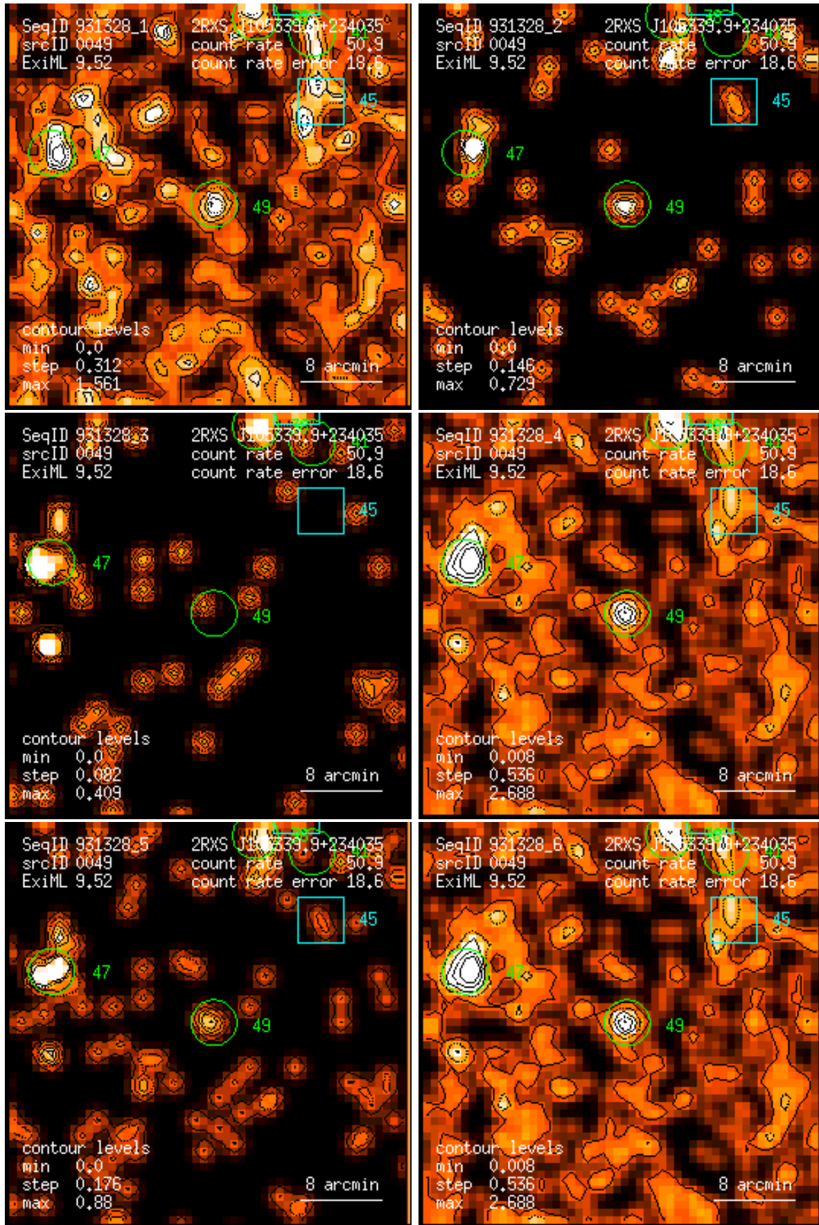
Figure 49: RASS 931328: detection 0049: band rate images, Gaussian filter: (1) PSPC channels 11 – 41, (2) 52 – 90, (3) 91 – 201, (4) 11 – 235, (5) 52 – 201, (6) 11 – 201. Broad band rates in counts/ks. Band rate contour levels in counts/ks/arcmin 2 .
